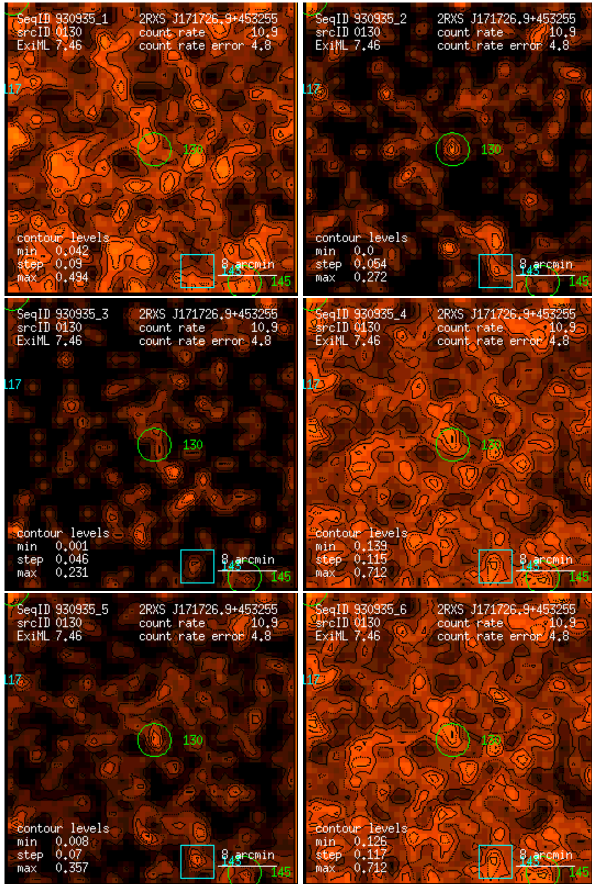
Figure 130: RASS 930935: detection 0130: band rate images, Gaussian filter: (1) PSPC channels 11 – 41, (2) 52 – 90, (3) 91 – 201, (4) 11 – 235, (5) 52 – 201, (6) 11 – 201. Broad band rates in counts/ks. Band rate contour levels in counts/ks/arcmin 2 .
