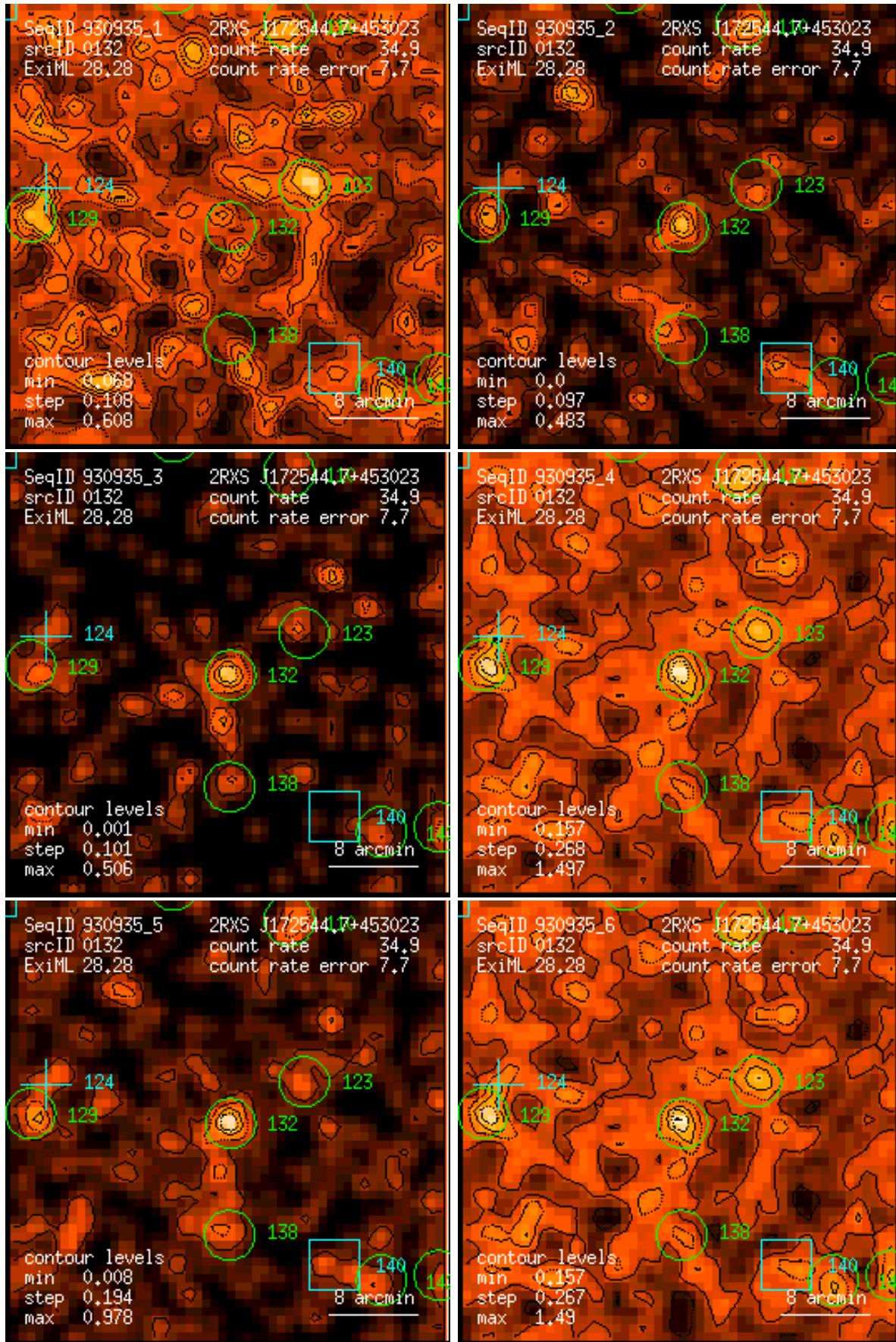
Figure 132: RASS 930935: detection 0132: band rate images, Gaussian filter: (1) PSPC channels 11 – 41, (2) 52 – 90, (3) 91 – 201, (4) 11 – 235, (5) 52 – 201, (6) 11 – 201. Broad band rates in counts/ks. Band rate contour levels in counts/ks/arcmin 2 .
