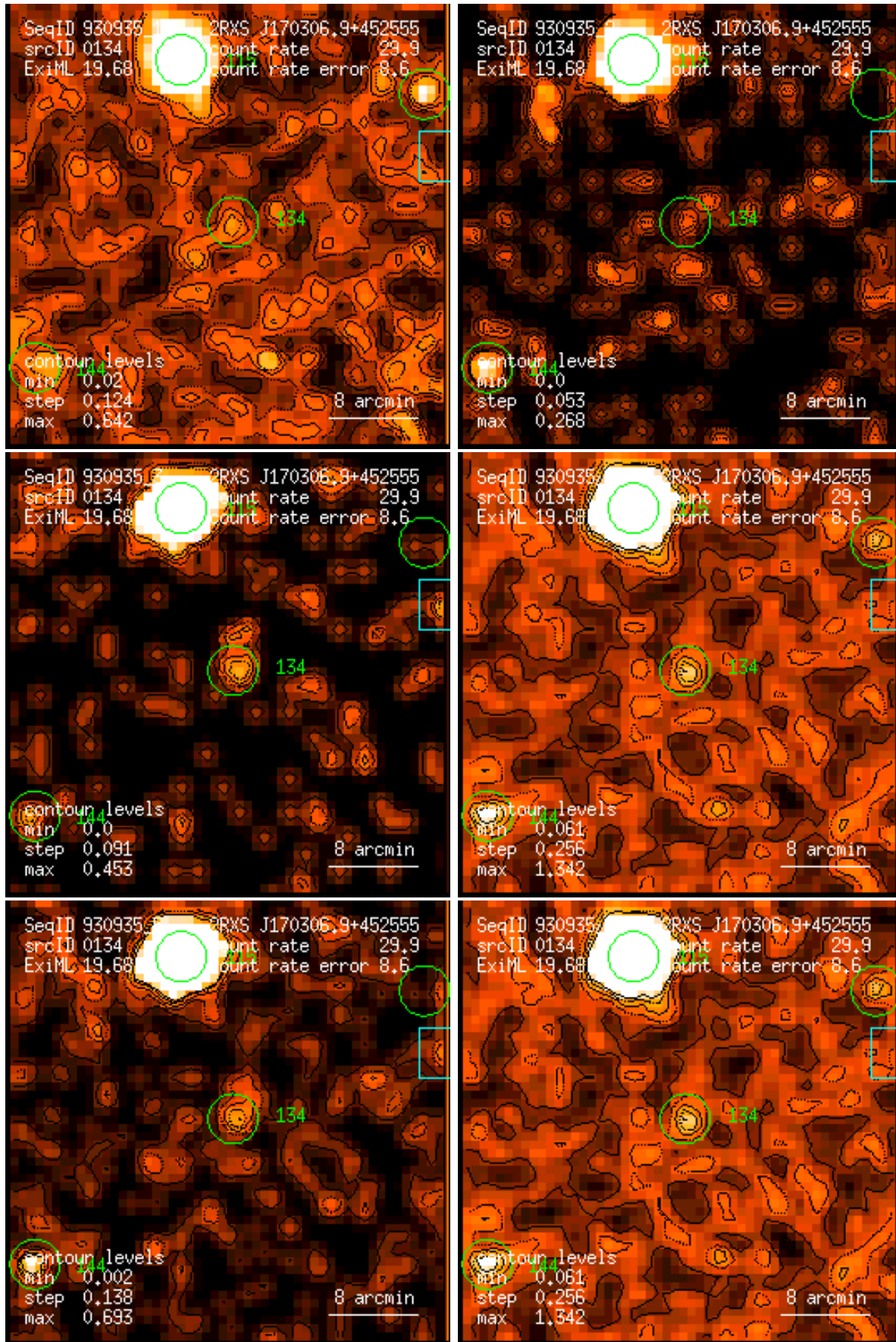
Figure 134: RASS 930935: detection 0134: band rate images, Gaussian filter: (1) PSPC channels 11 – 41, (2) 52 – 90, (3) 91 – 201, (4) 11 – 235, (5) 52 – 201, (6) 11 – 201. Broad band rates in counts/ks. Band rate contour levels in counts/ks/arcmin 2 .
