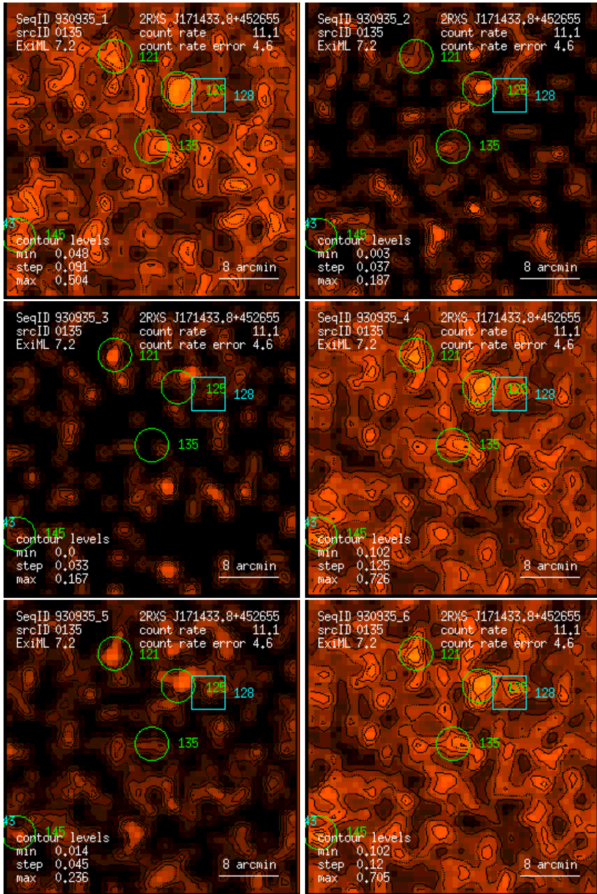
Figure 135: RASS 930935: detection 0135: band rate images, Gaussian filter: (1) PSPC channels 11 – 41, (2) 52 – 90, (3) 91 – 201, (4) 11 – 235, (5) 52 – 201, (6) 11 – 201. Broad band rates in counts/ks. Band rate contour levels in counts/ks/arcmin 2 .
