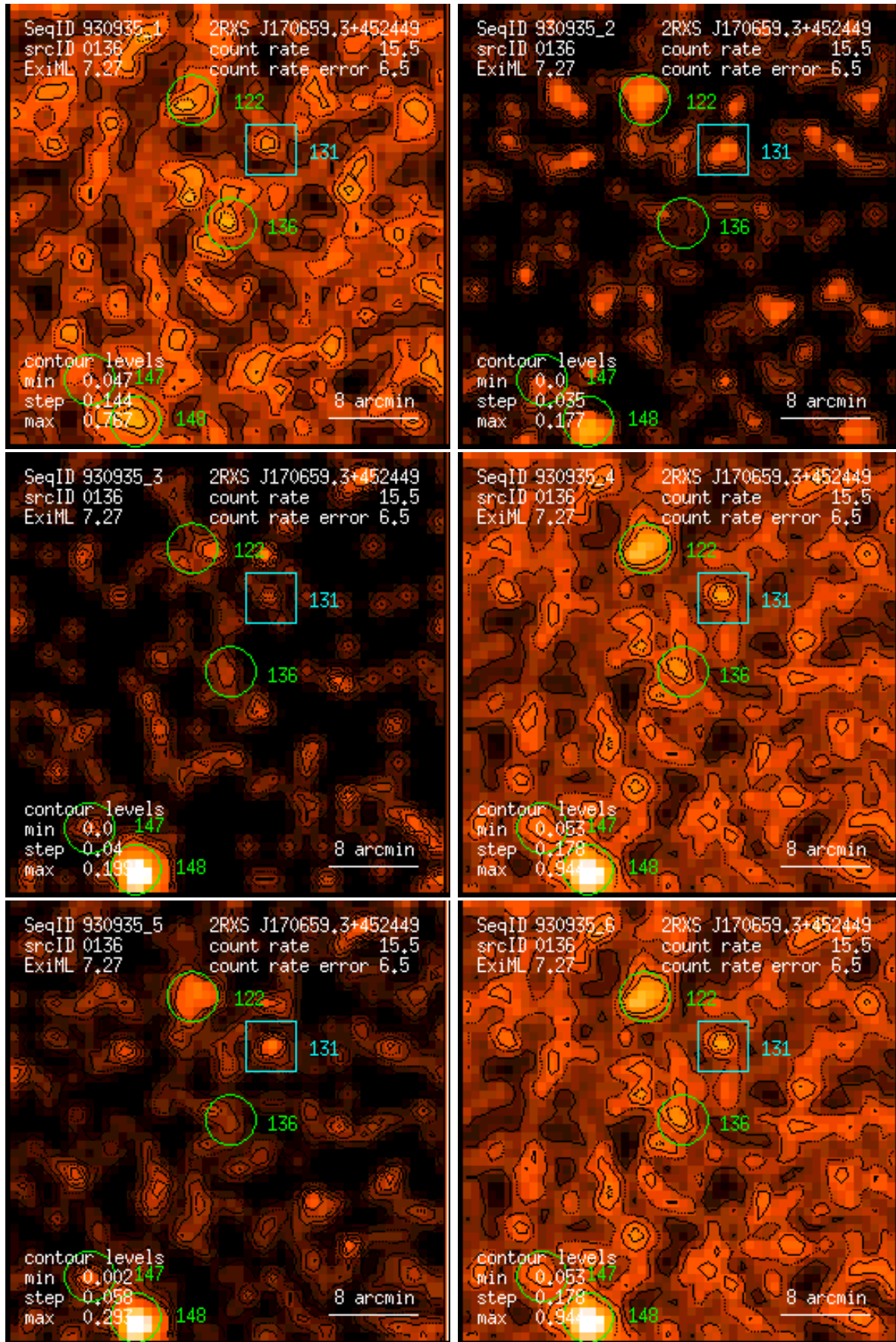
Figure 136: RASS 930935: detection 0136: band rate images, Gaussian filter: (1) PSPC channels 11 – 41, (2) 52 – 90, (3) 91 – 201, (4) 11 – 235, (5) 52 – 201, (6) 11 – 201. Broad band rates in counts/ks. Band rate contour levels in counts/ks/arcmin 2 .
