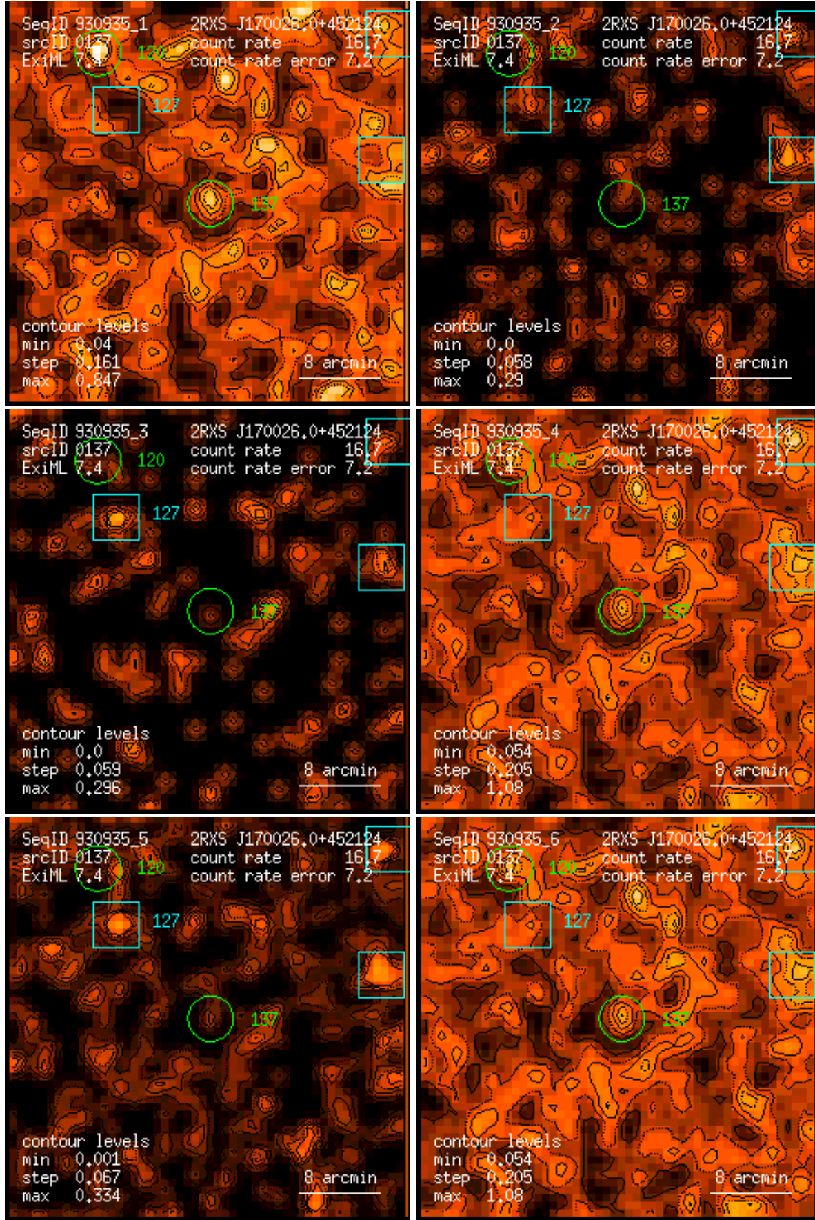
Figure 137: RASS 930935: detection 0137: band rate images, Gaussian filter: (1) PSPC channels 11 – 41, (2) 52 – 90, (3) 91 – 201, (4) 11 – 235, (5) 52 – 201, (6) 11 – 201. Broad band rates in counts/ks. Band rate contour levels in counts/ks/arcmin 2 .
