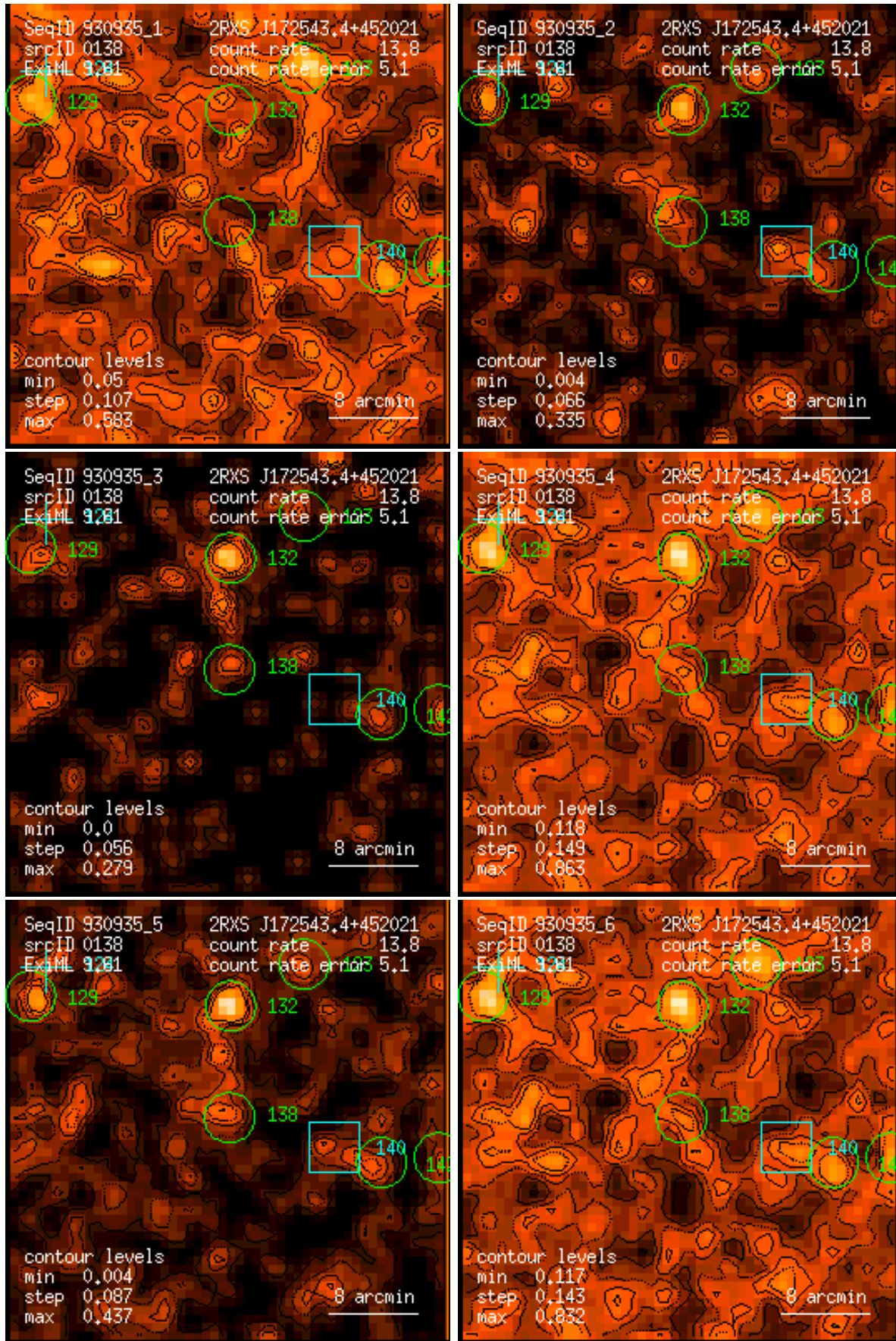
Figure 138: RASS 930935: detection 0138: band rate images, Gaussian filter: (1) PSPC channels 11 – 41, (2) 52 – 90, (3) 91 – 201, (4) 11 – 235, (5) 52 – 201, (6) 11 – 201. Broad band rates in counts/ks. Band rate contour levels in counts/ks/arcmin 2 .
