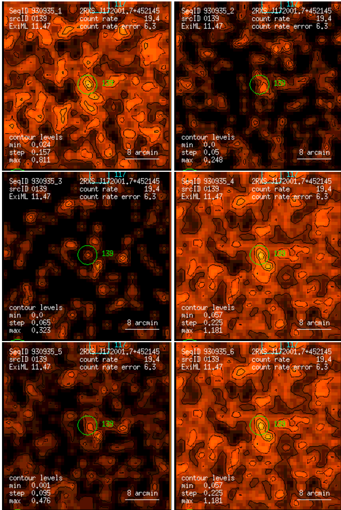
Figure 139: RASS 930935: detection 0139: band rate images, Gaussian filter: (1) PSPC channels 11 – 41, (2) 52 – 90, (3) 91 – 201, (4) 11 – 235, (5) 52 – 201, (6) 11 – 201. Broad band rates in counts/ks. Band rate contour levels in counts/ks/arcmin 2 .
