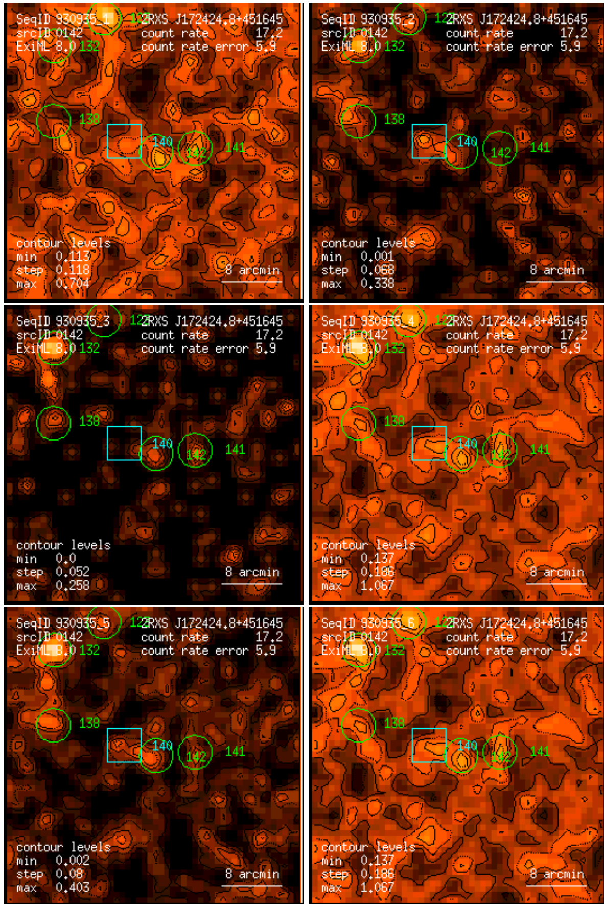
Figure 142: RASS 930935: detection 0142: band rate images, Gaussian filter: (1) PSPC channels 11 – 41, (2) 52 – 90, (3) 91 – 201, (4) 11 – 235, (5) 52 – 201, (6) 11 – 201. Broad band rates in counts/ks. Band rate contour levels in counts/ks/arcmin 2 .
