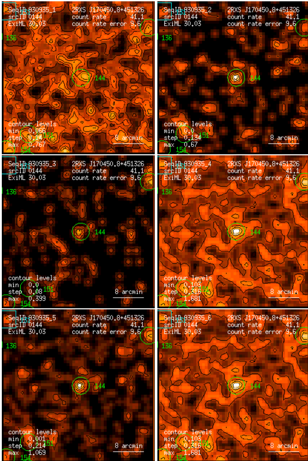
Figure 144: RASS 930935: detection 0144: band rate images, Gaussian filter: (1) PSPC channels 11 – 41, (2) 52 – 90, (3) 91 – 201, (4) 11 – 235, (5) 52 – 201, (6) 11 – 201. Broad band rates in counts/ks. Band rate contour levels in counts/ks/arcmin 2 .
