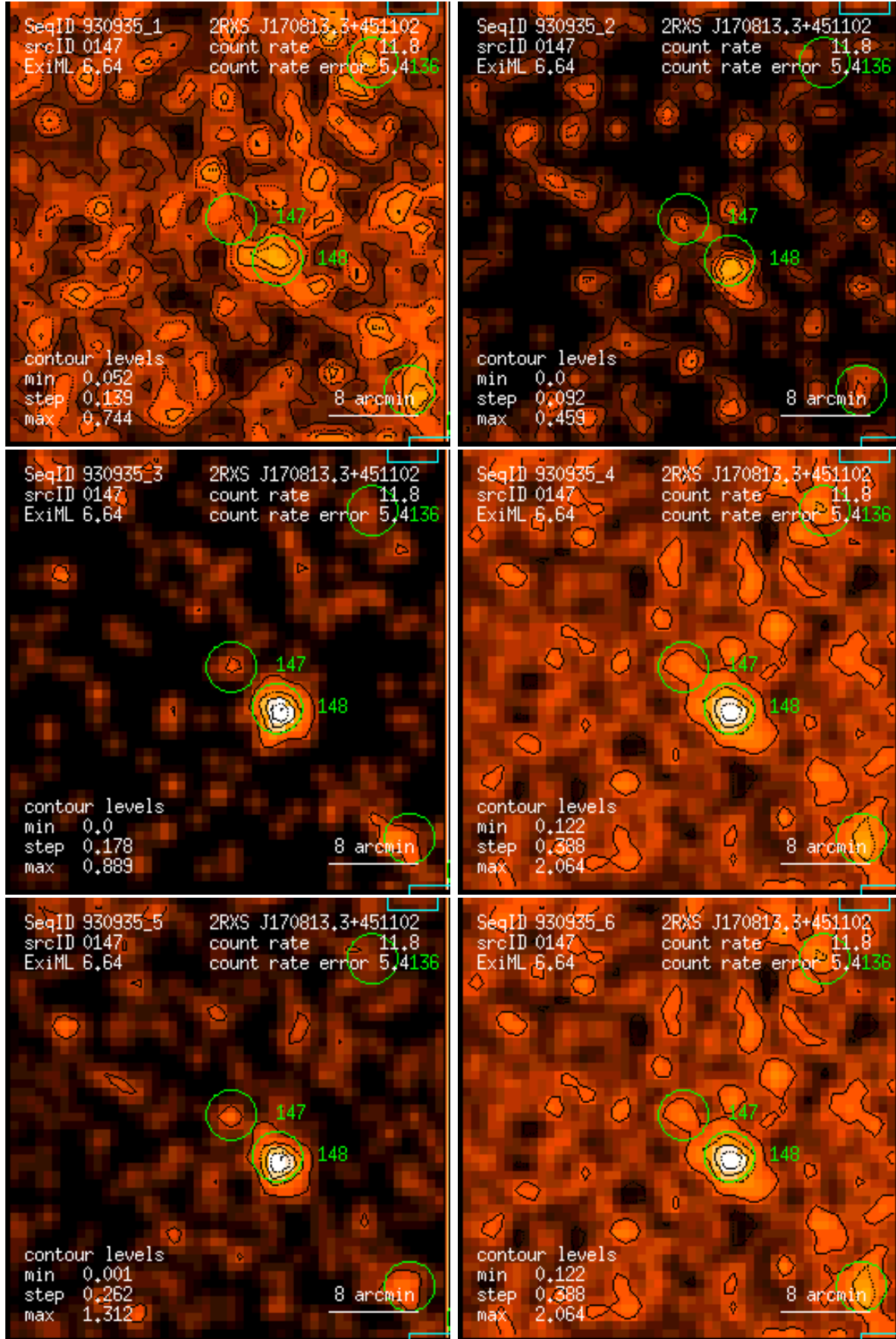
Figure 147: RASS 930935: detection 0147: band rate images, Gaussian filter: (1) PSPC channels 11 – 41, (2) 52 – 90, (3) 91 – 201, (4) 11 – 235, (5) 52 – 201, (6) 11 – 201. Broad band rates in counts/ks. Band rate contour levels in counts/ks/arcmin 2 .
