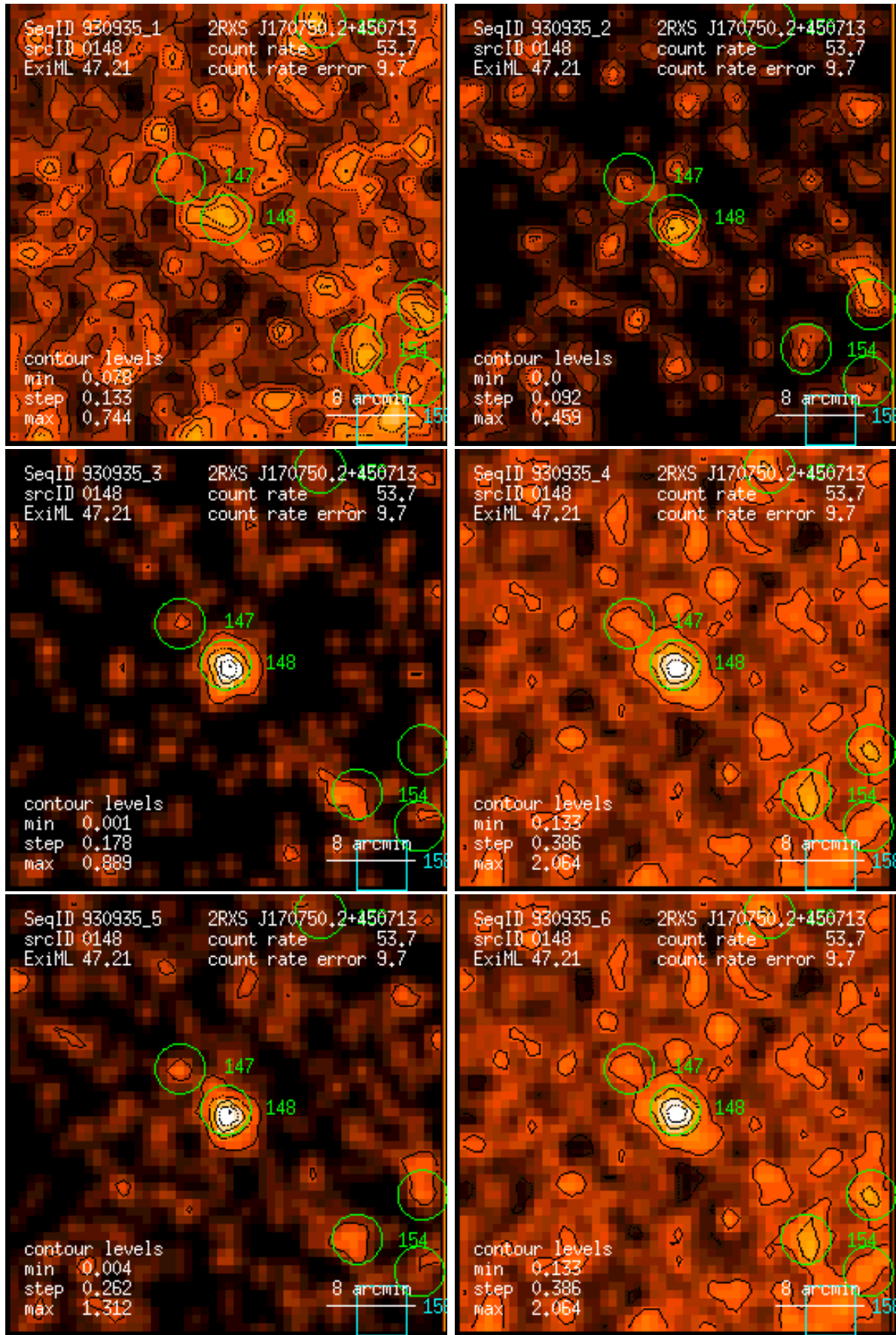
Figure 148: RASS 930935: detection 0148: band rate images, Gaussian filter: (1) PSPC channels 11 – 41, (2) 52 – 90, (3) 91 – 201, (4) 11 – 235, (5) 52 – 201, (6) 11 – 201. Broad band rates in counts/ks. Band rate contour levels in counts/ks/arcmin 2 .
