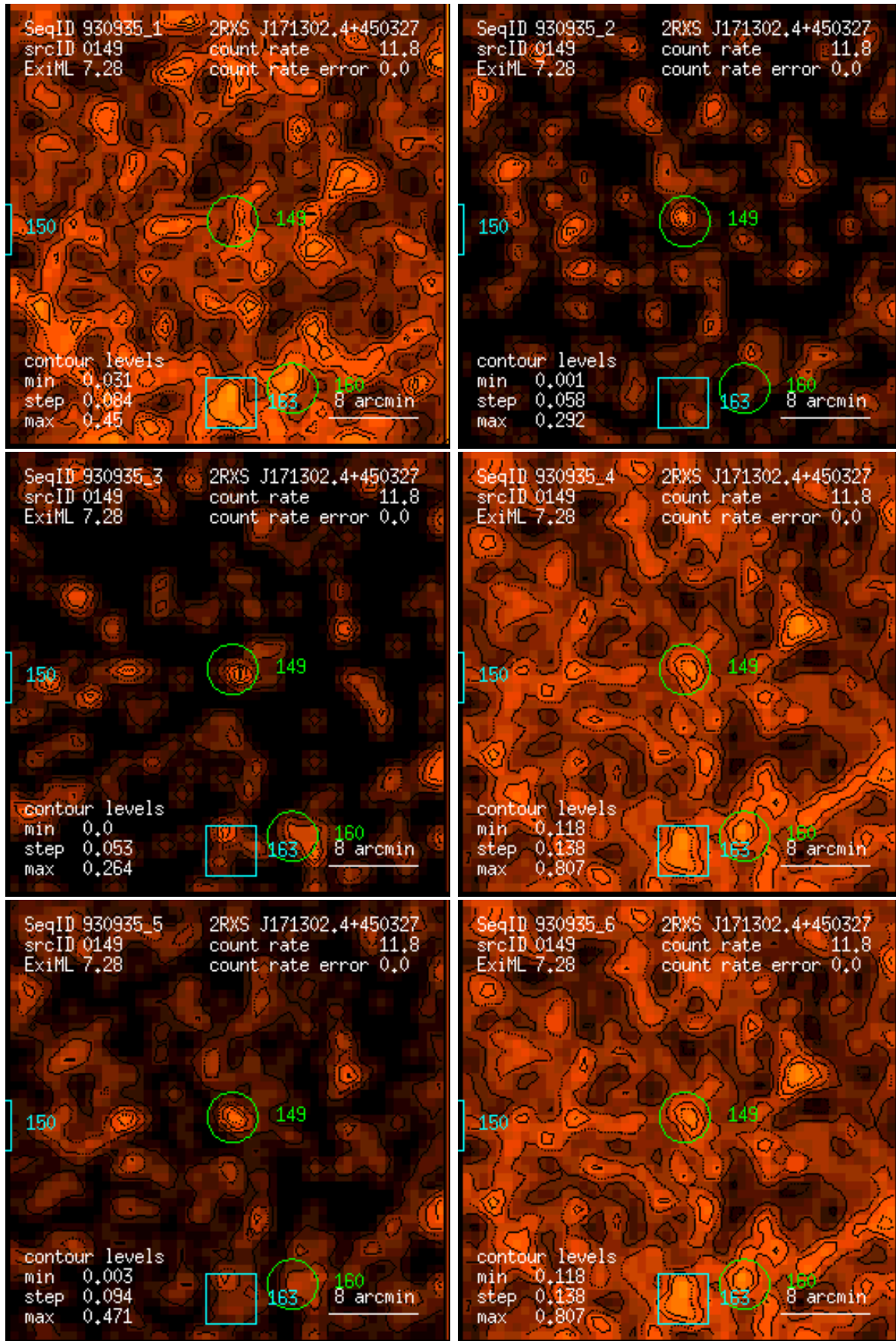
Figure 149: RASS 930935: detection 0149: band rate images, Gaussian filter: (1) PSPC channels 11 – 41, (2) 52 – 90, (3) 91 – 201, (4) 11 – 235, (5) 52 – 201, (6) 11 – 201. Broad band rates in counts/ks. Band rate contour levels in counts/ks/arcmin 2 .
