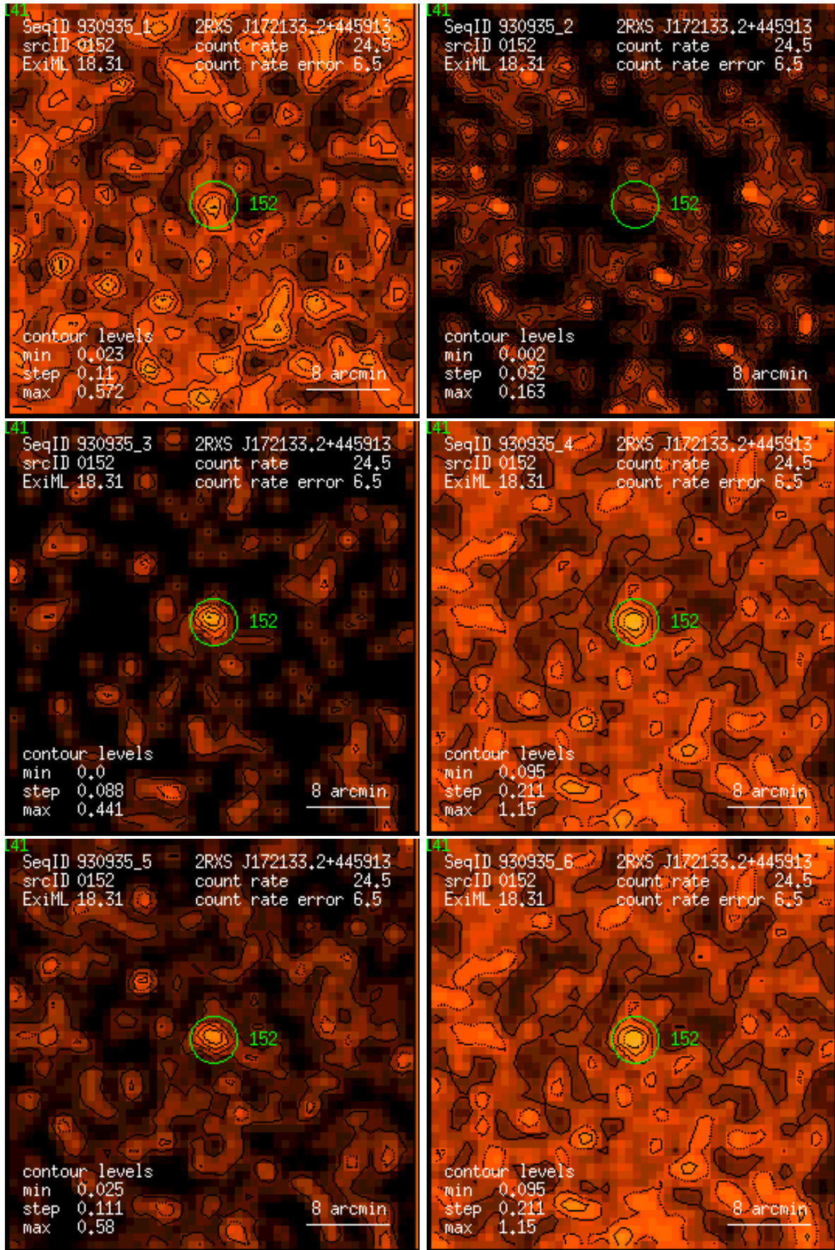
Figure 152: RASS 930935: detection 0152: band rate images, Gaussian filter: (1) PSPC channels 11 – 41, (2) 52 – 90, (3) 91 – 201, (4) 11 – 235, (5) 52 – 201, (6) 11 – 201. Broad band rates in counts/ks. Band rate contour levels in counts/ks/arcmin 2 .
