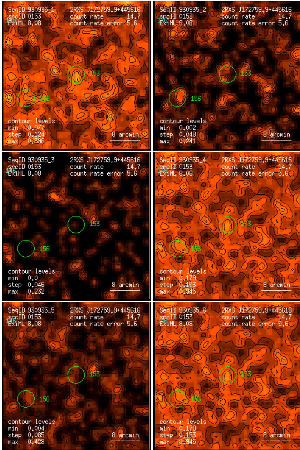
Figure 153: RASS 930935: detection 0153: band rate images, Gaussian filter: (1) PSPC channels 11 – 41, (2) 52 – 90, (3) 91 – 201, (4) 11 – 235, (5) 52 – 201, (6) 11 – 201. Broad band rates in counts/ks. Band rate contour levels in counts/ks/arcmin 2 .
