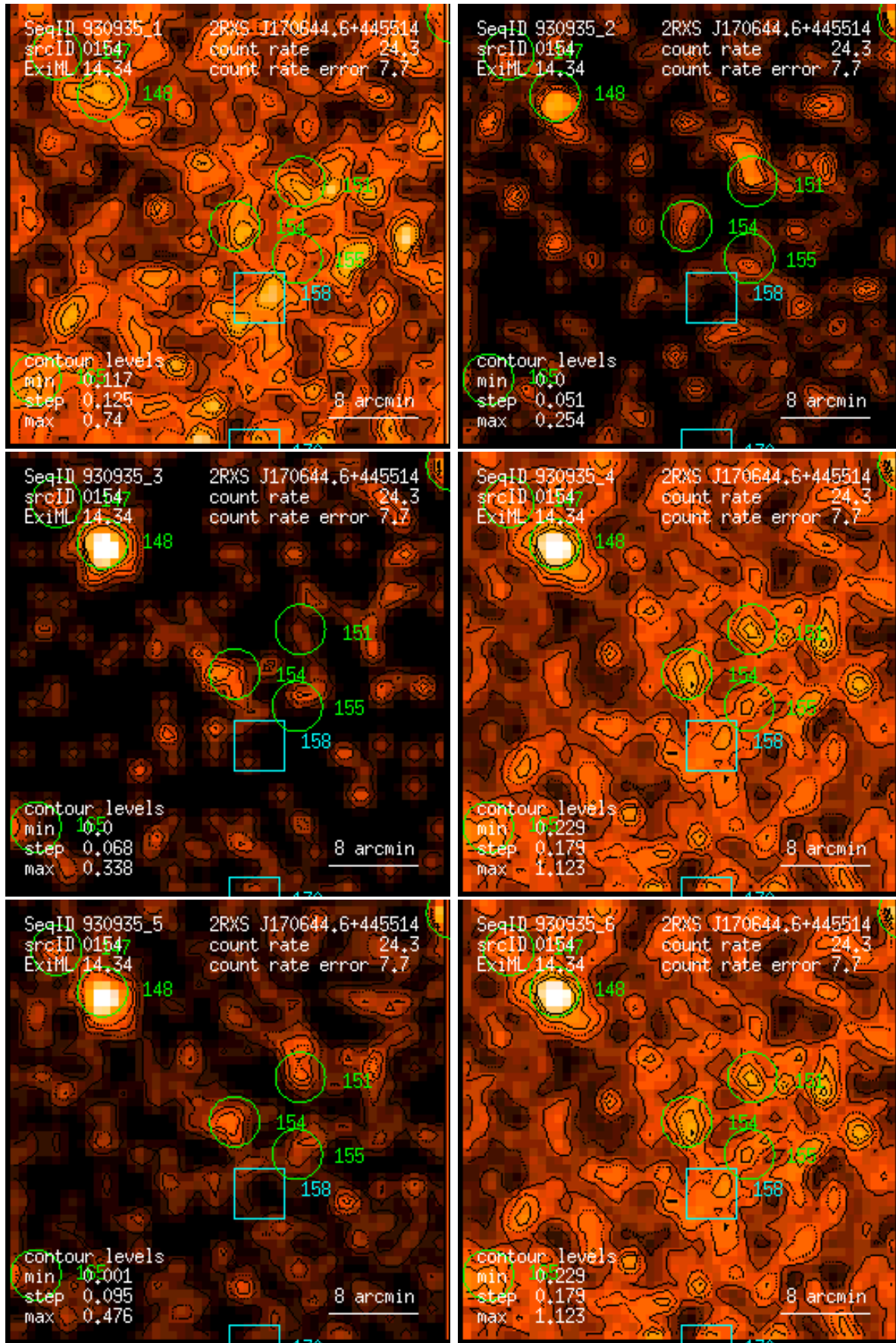
Figure 154: RASS 930935: detection 0154: band rate images, Gaussian filter: (1) PSPC channels 11 – 41, (2) 52 – 90, (3) 91 – 201, (4) 11 – 235, (5) 52 – 201, (6) 11 – 201. Broad band rates in counts/ks. Band rate contour levels in counts/ks/arcmin 2 .
