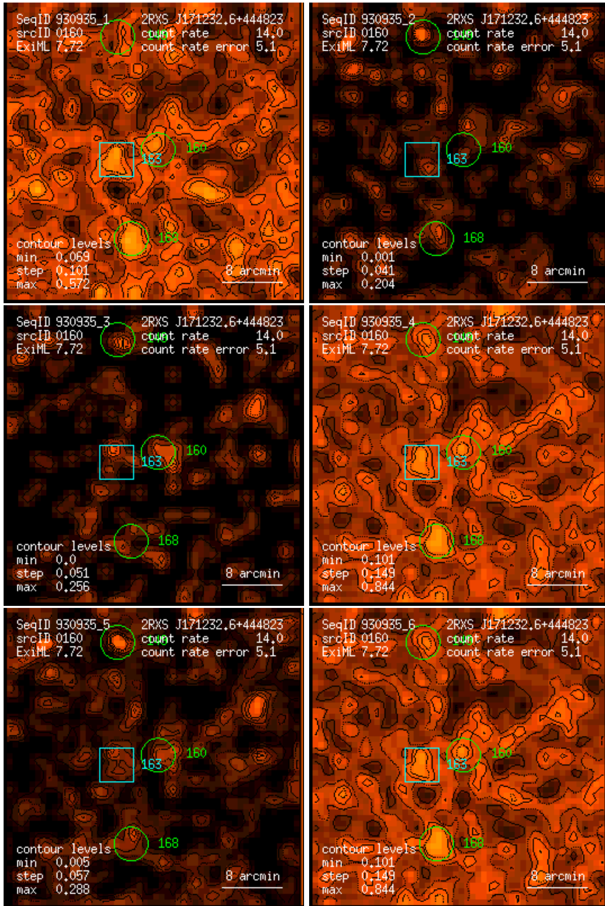
Figure 160: RASS 930935: detection 0160: band rate images, Gaussian filter: (1) PSPC channels 11 – 41, (2) 52 – 90, (3) 91 – 201, (4) 11 – 235, (5) 52 – 201, (6) 11 – 201. Broad band rates in counts/ks. Band rate contour levels in counts/ks/arcmin 2 .
