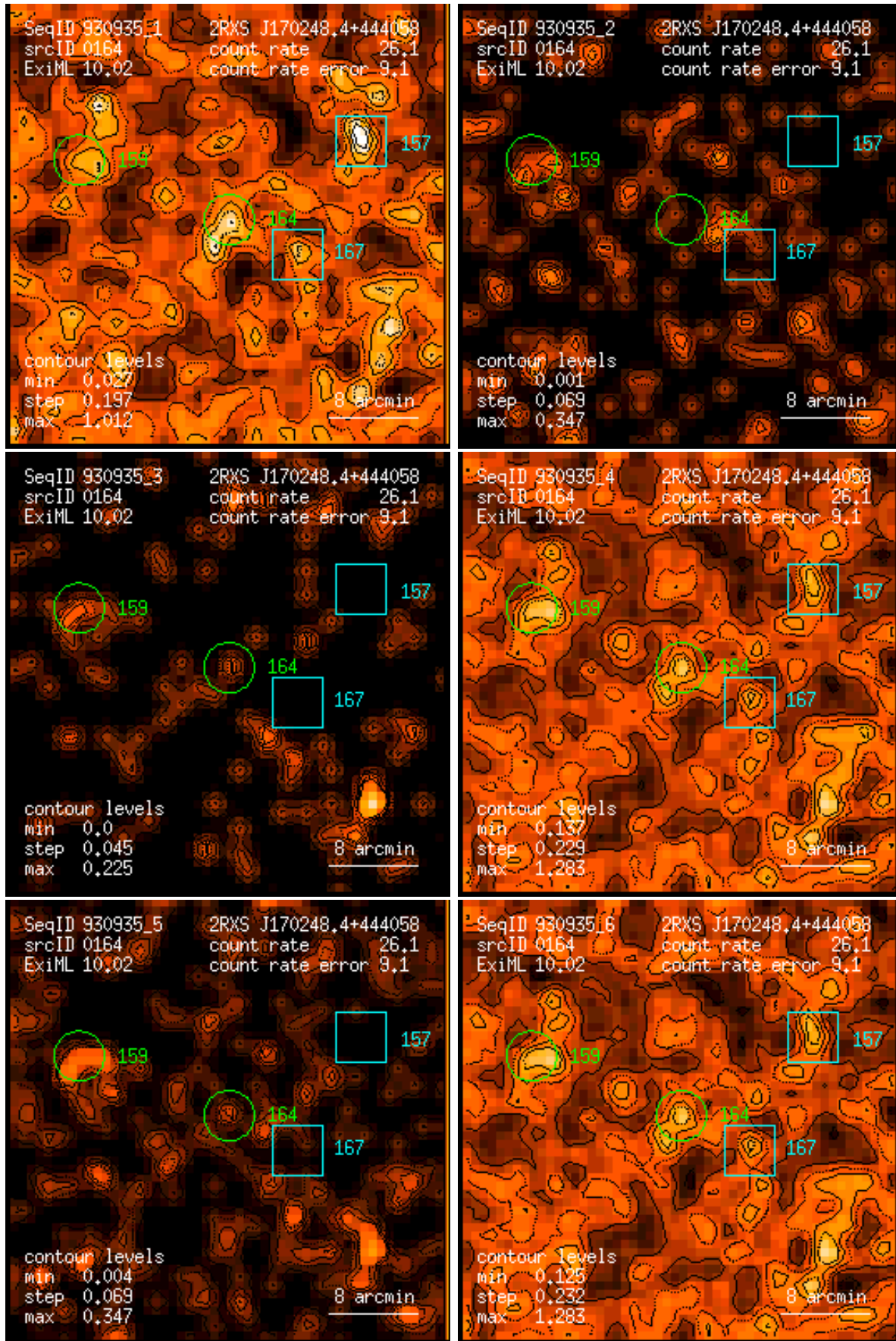
Figure 164: RASS 930935: detection 0164: band rate images, Gaussian filter: (1) PSPC channels 11 – 41, (2) 52 – 90, (3) 91 – 201, (4) 11 – 235, (5) 52 – 201, (6) 11 – 201. Broad band rates in counts/ks. Band rate contour levels in counts/ks/arcmin 2 .
