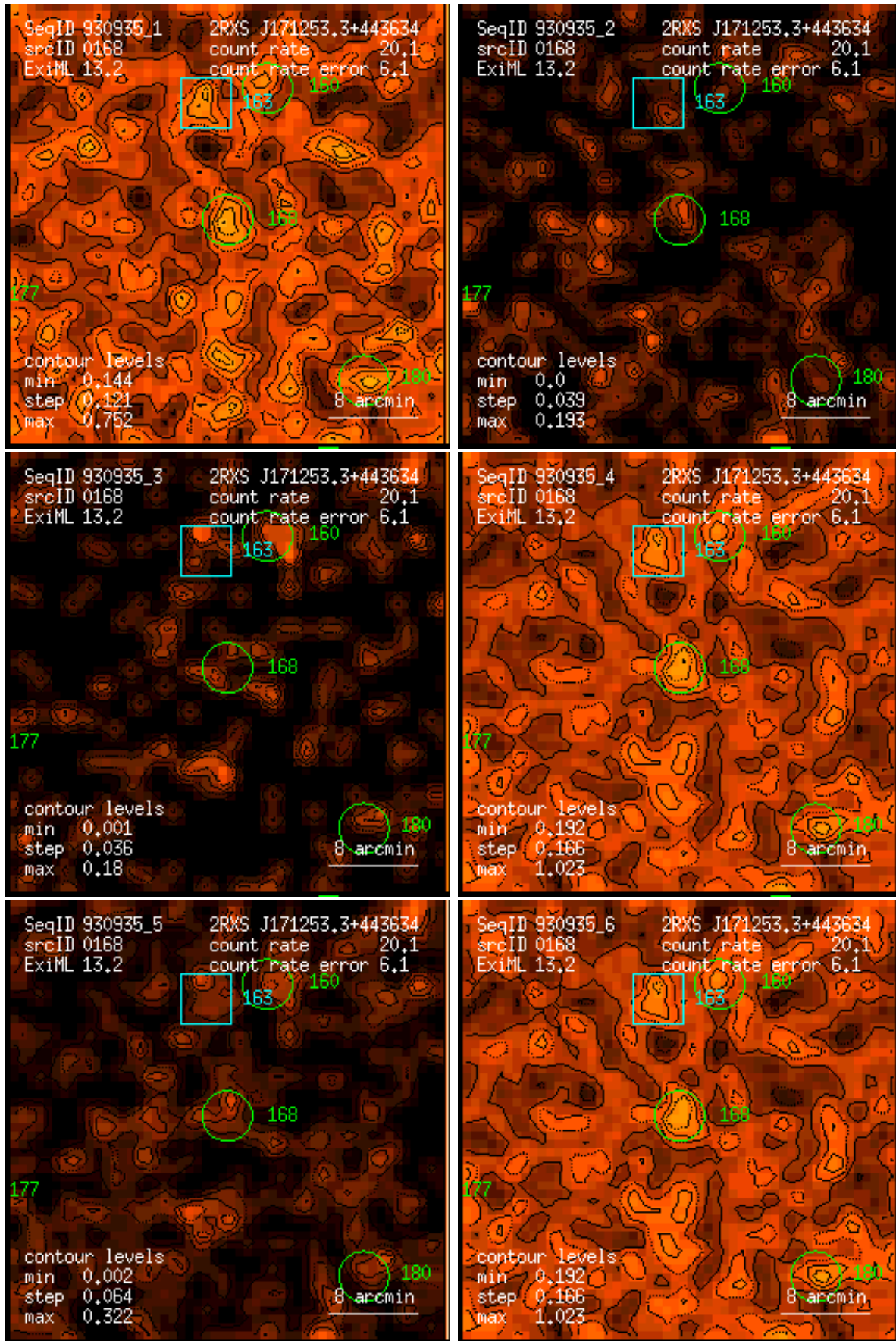
Figure 168: RASS 930935: detection 0168: band rate images, Gaussian filter: (1) PSPC channels 11 – 41, (2) 52 – 90, (3) 91 – 201, (4) 11 – 235, (5) 52 – 201, (6) 11 – 201. Broad band rates in counts/ks. Band rate contour levels in counts/ks/arcmin 2 .
