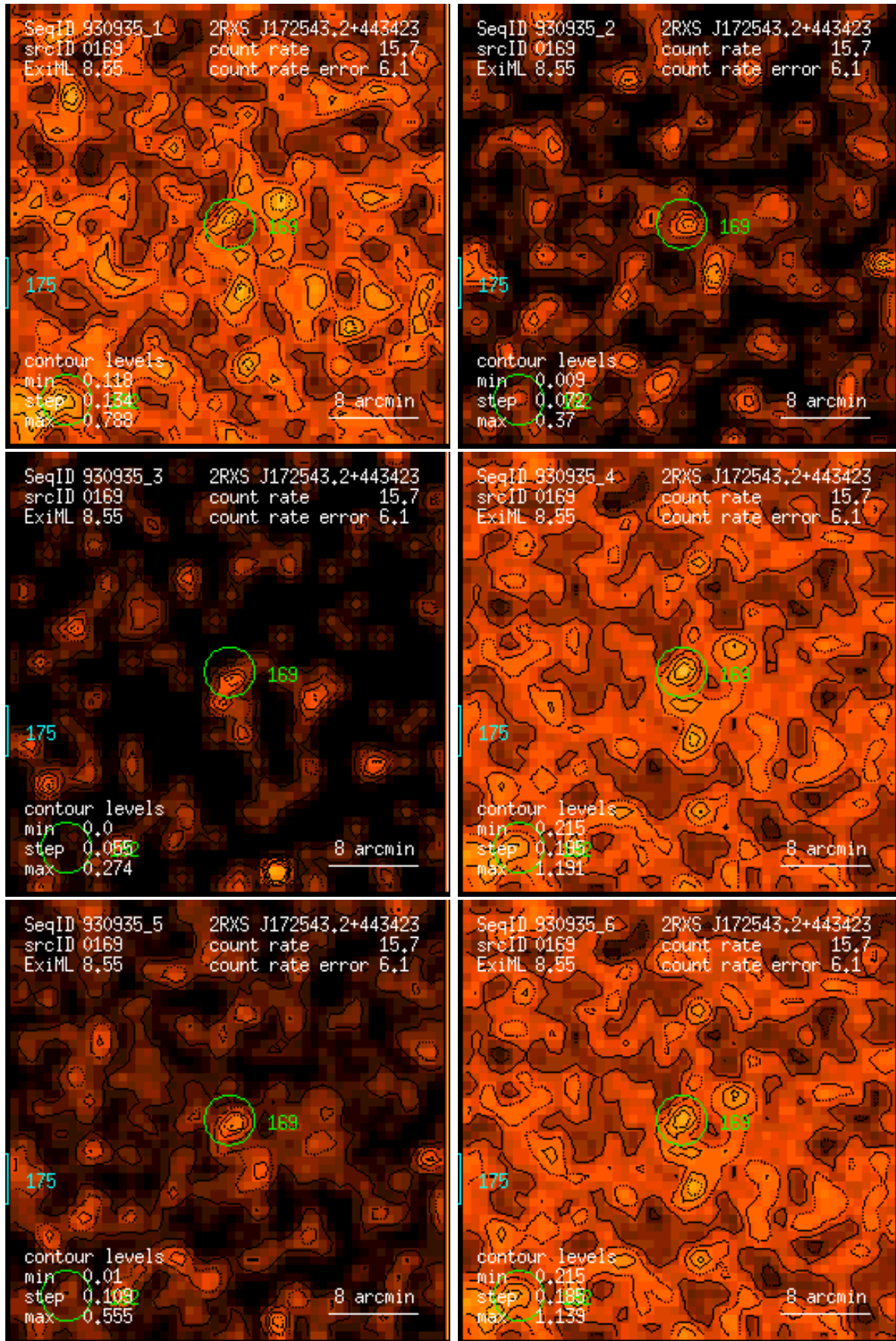
Figure 169: RASS 930935: detection 0169: band rate images, Gaussian filter: (1) PSPC channels 11 – 41, (2) 52 – 90, (3) 91 – 201, (4) 11 – 235, (5) 52 – 201, (6) 11 – 201. Broad band rates in counts/ks. Band rate contour levels in counts/ks/arcmin 2 .
