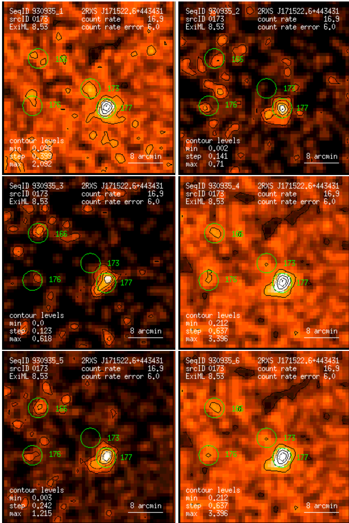
Figure 173: RASS 930935: detection 0173: band rate images, Gaussian filter: (1) PSPC channels 11 – 41, (2) 52 – 90, (3) 91 – 201, (4) 11 – 235, (5) 52 – 201, (6) 11 – 201. Broad band rates in counts/ks. Band rate contour levels in counts/ks/arcmin 2 .
