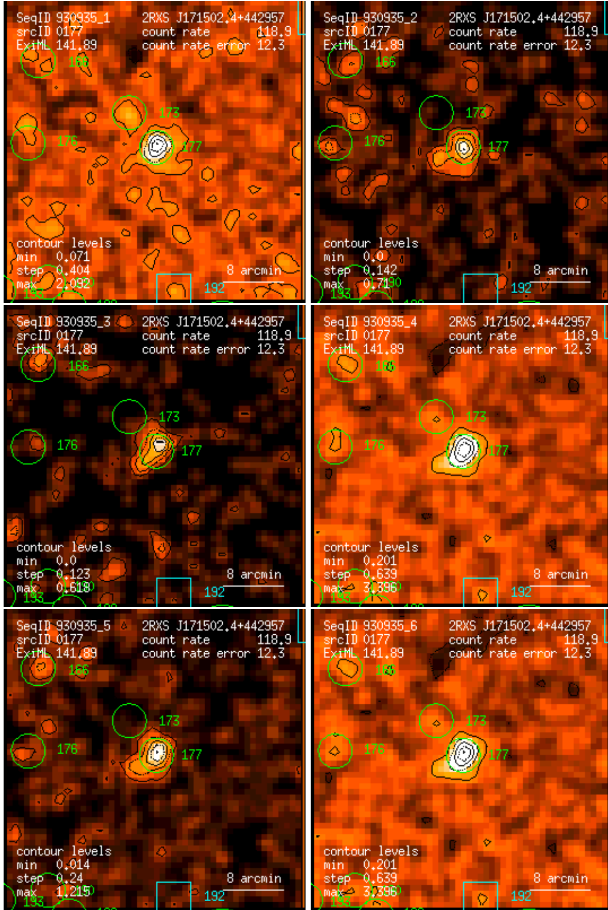
Figure 177: RASS 930935: detection 0177: band rate images, Gaussian filter: (1) PSPC channels 11 – 41, (2) 52 – 90, (3) 91 – 201, (4) 11 – 235, (5) 52 – 201, (6) 11 – 201. Broad band rates in counts/ks. Band rate contour levels in counts/ks/arcmin 2 .
