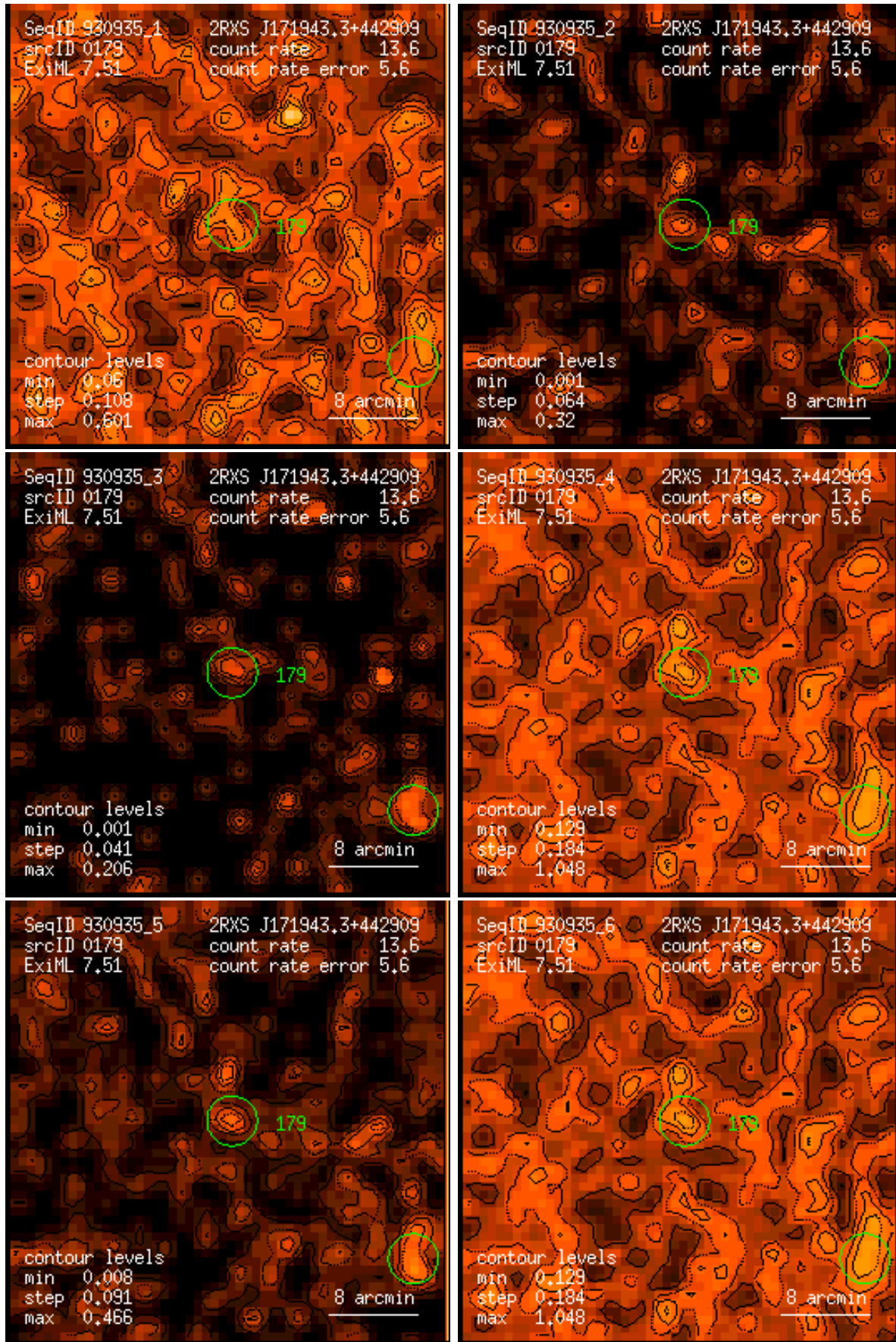
Figure 179: RASS 930935: detection 0179: band rate images, Gaussian filter: (1) PSPC channels 11 – 41, (2) 52 – 90, (3) 91 – 201, (4) 11 – 235, (5) 52 – 201, (6) 11 – 201. Broad band rates in counts/ks. Band rate contour levels in counts/ks/arcmin 2 .
