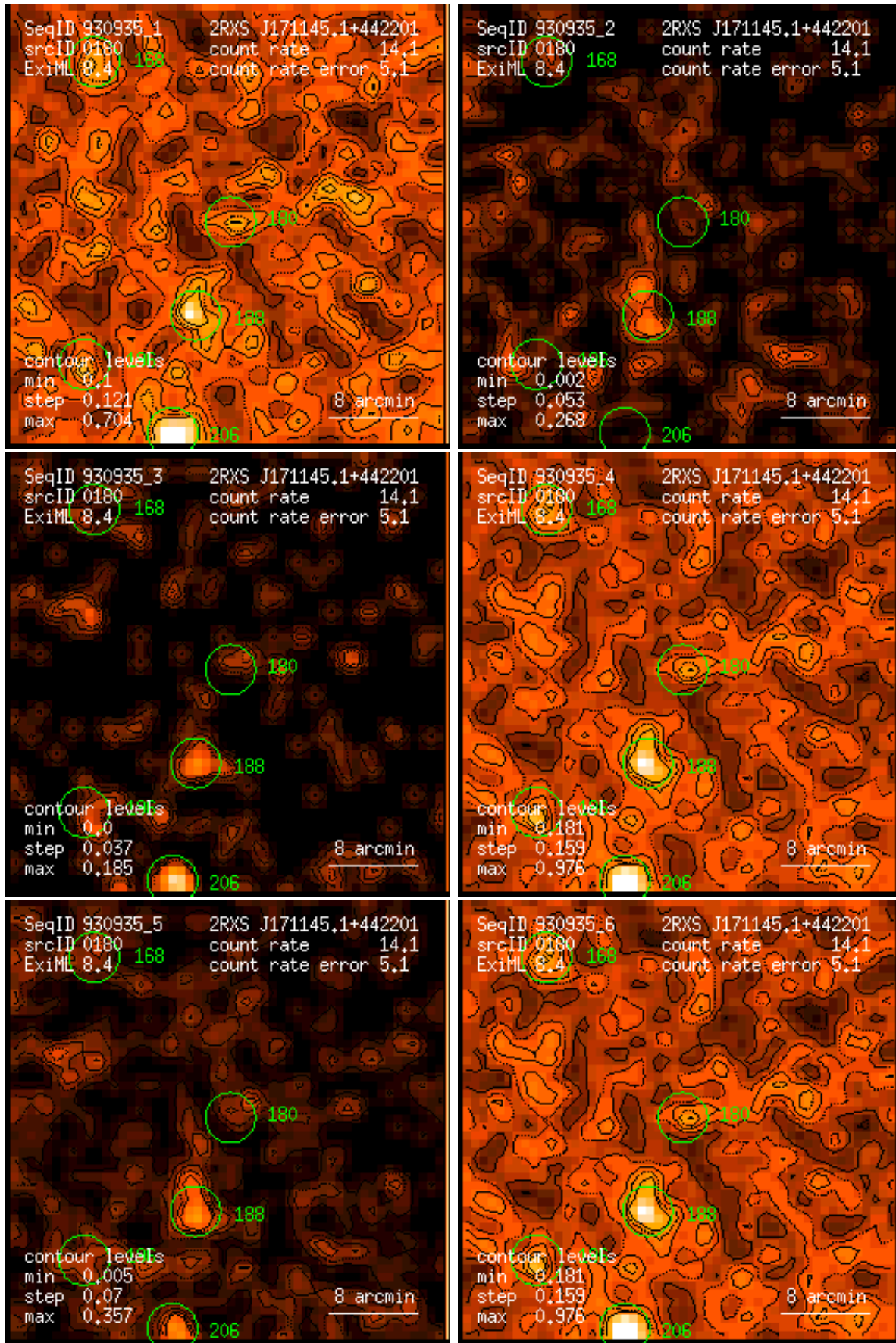
Figure 180: RASS 930935: detection 0180: band rate images, Gaussian filter: (1) PSPC channels 11 – 41, (2) 52 – 90, (3) 91 – 201, (4) 11 – 235, (5) 52 – 201, (6) 11 – 201. Broad band rates in counts/ks. Band rate contour levels in counts/ks/arcmin 2 .
