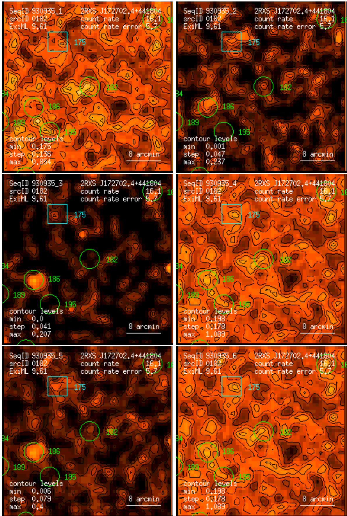
Figure 182: RASS 930935: detection 0182: band rate images, Gaussian filter: (1) PSPC channels 11 – 41, (2) 52 – 90, (3) 91 – 201, (4) 11 – 235, (5) 52 – 201, (6) 11 – 201. Broad band rates in counts/ks. Band rate contour levels in counts/ks/arcmin 2 .
