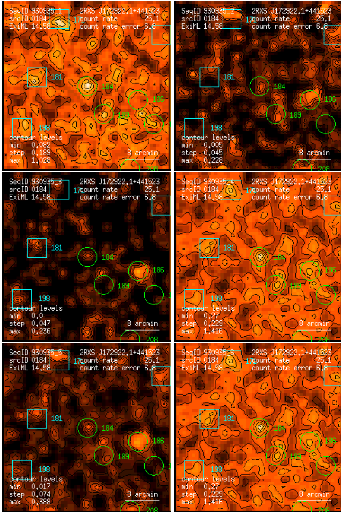
Figure 184: RASS 930935: detection 0184: band rate images, Gaussian filter: (1) PSPC channels 11 – 41, (2) 52 – 90, (3) 91 – 201, (4) 11 – 235, (5) 52 – 201, (6) 11 – 201. Broad band rates in counts/ks. Band rate contour levels in counts/ks/arcmin 2 .
