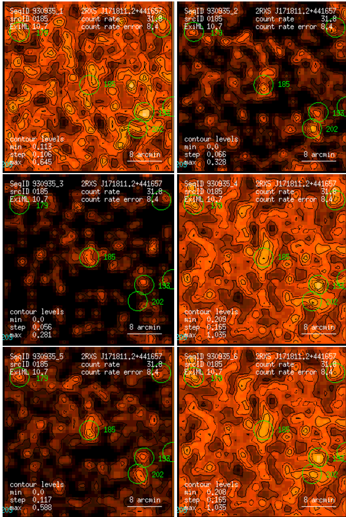
Figure 185: RASS 930935: detection 0185: band rate images, Gaussian filter: (1) PSPC channels 11 – 41, (2) 52 – 90, (3) 91 – 201, (4) 11 – 235, (5) 52 – 201, (6) 11 – 201. Broad band rates in counts/ks. Band rate contour levels in counts/ks/arcmin 2 .
