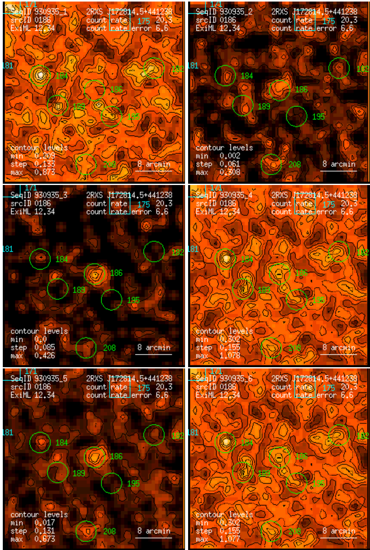
Figure 186: RASS 930935: detection 0186: band rate images, Gaussian filter: (1) PSPC channels 11 – 41, (2) 52 – 90, (3) 91 – 201, (4) 11 – 235, (5) 52 – 201, (6) 11 – 201. Broad band rates in counts/ks. Band rate contour levels in counts/ks/arcmin 2 .
