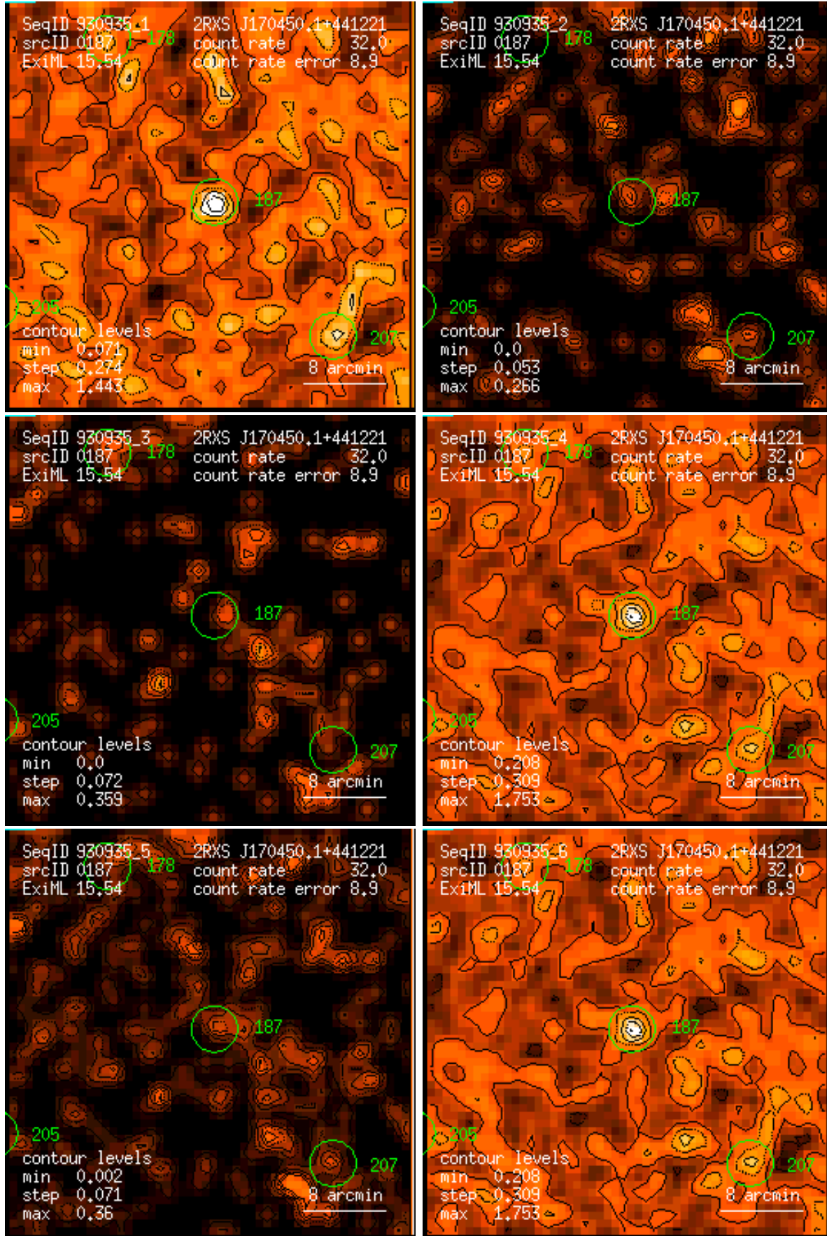
Figure 187: RASS 930935: detection 0187: band rate images, Gaussian filter: (1) PSPC channels 11 – 41, (2) 52 – 90, (3) 91 – 201, (4) 11 – 235, (5) 52 – 201, (6) 11 – 201. Broad band rates in counts/ks. Band rate contour levels in counts/ks/arcmin 2 .
