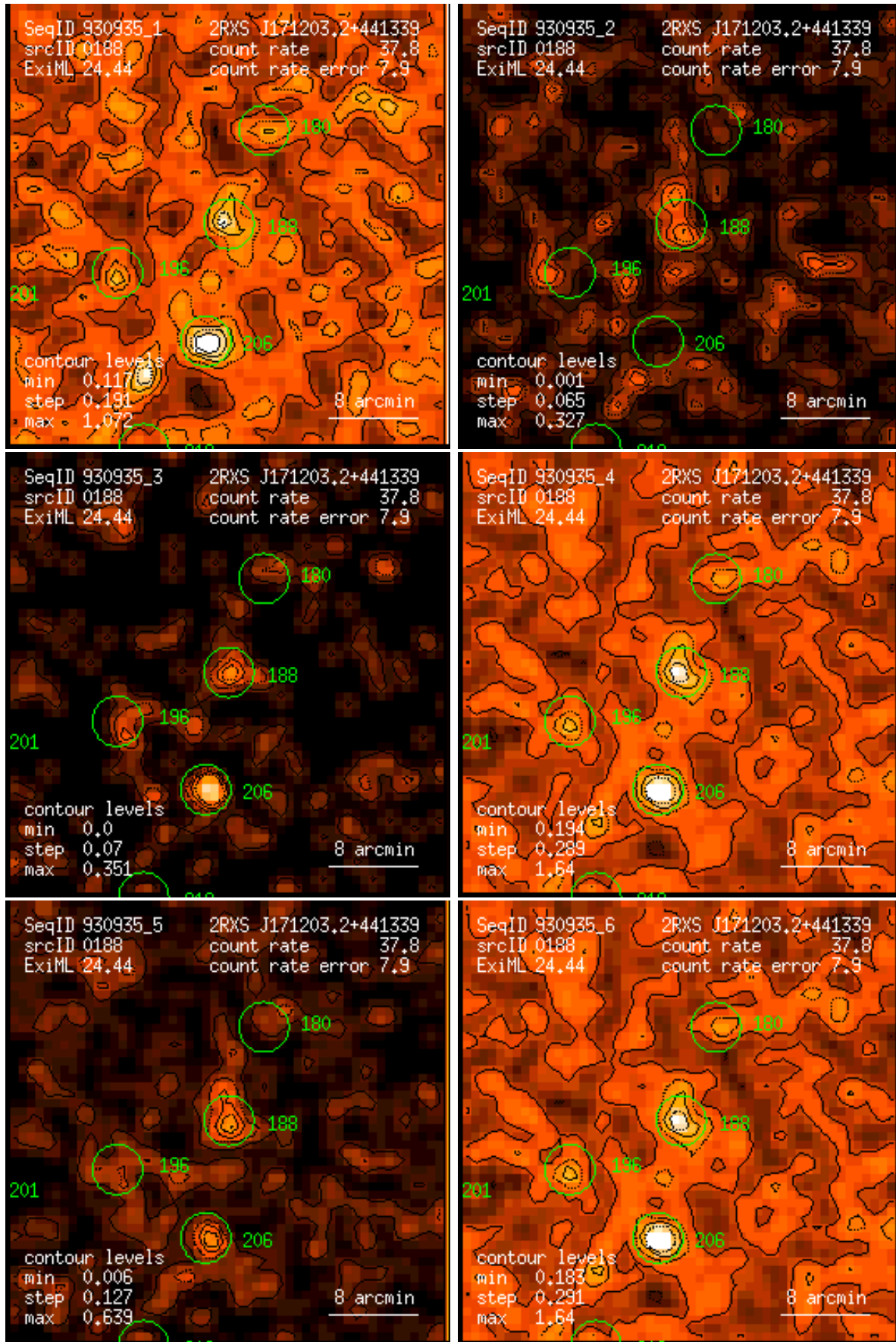
Figure 188: RASS 930935: detection 0188: band rate images, Gaussian filter: (1) PSPC channels 11 – 41, (2) 52 – 90, (3) 91 – 201, (4) 11 – 235, (5) 52 – 201, (6) 11 – 201. Broad band rates in counts/ks. Band rate contour levels in counts/ks/arcmin 2 .
