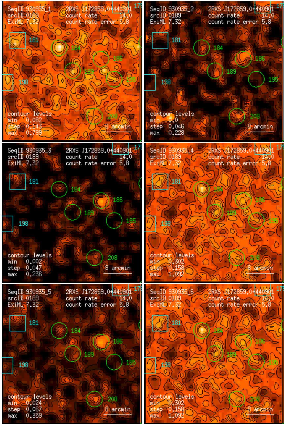
Figure 189: RASS 930935: detection 0189: band rate images, Gaussian filter: (1) PSPC channels 11 – 41, (2) 52 – 90, (3) 91 – 201, (4) 11 – 235, (5) 52 – 201, (6) 11 – 201. Broad band rates in counts/ks. Band rate contour levels in counts/ks/arcmin 2 .
