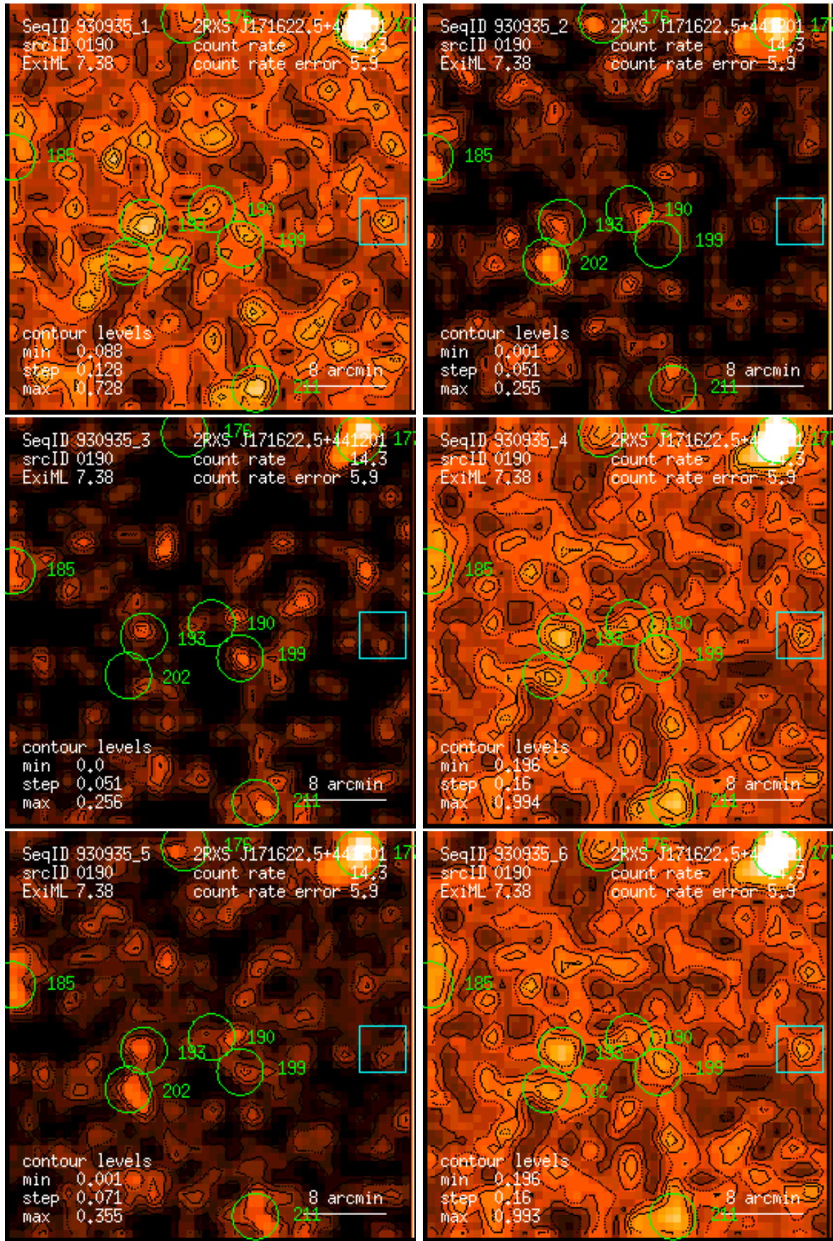
Figure 190: RASS 930935: detection 0190: band rate images, Gaussian filter: (1) PSPC channels 11 – 41, (2) 52 – 90, (3) 91 – 201, (4) 11 – 235, (5) 52 – 201, (6) 11 – 201. Broad band rates in counts/ks. Band rate contour levels in counts/ks/arcmin 2 .
