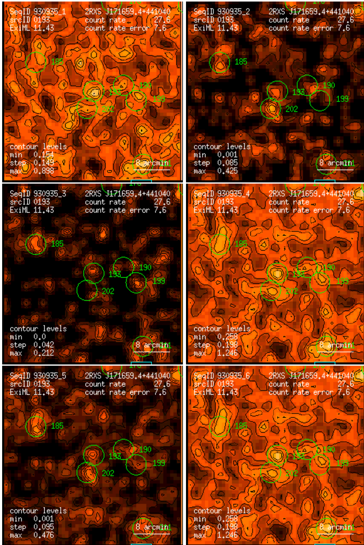
Figure 193: RASS 930935: detection 0193: band rate images, Gaussian filter: (1) PSPC channels 11 – 41, (2) 52 – 90, (3) 91 – 201, (4) 11 – 235, (5) 52 – 201, (6) 11 – 201. Broad band rates in counts/ks. Band rate contour levels in counts/ks/arcmin 2 .
