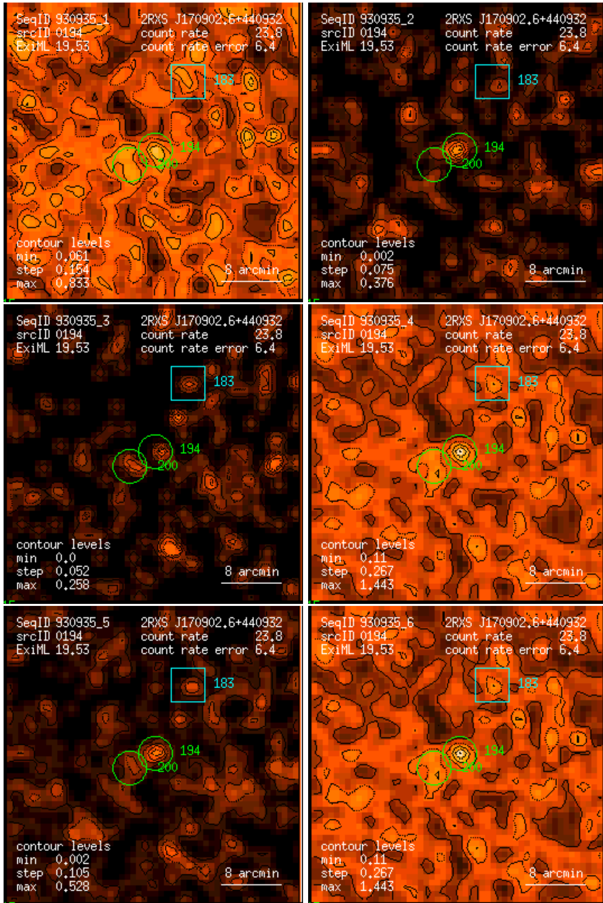
Figure 194: RASS 930935: detection 0194: band rate images, Gaussian filter: (1) PSPC channels 11 – 41, (2) 52 – 90, (3) 91 – 201, (4) 11 – 235, (5) 52 – 201, (6) 11 – 201. Broad band rates in counts/ks. Band rate contour levels in counts/ks/arcmin 2 .
