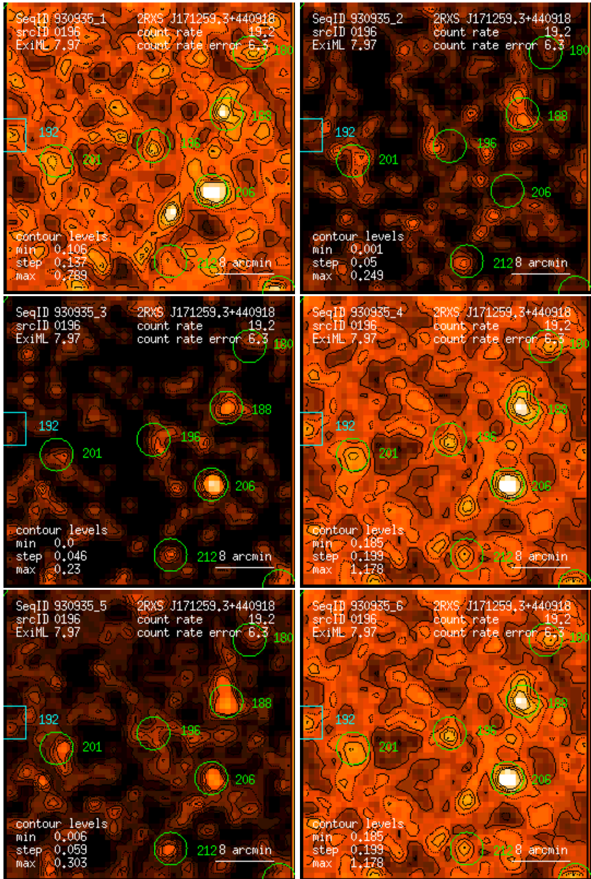
Figure 196: RASS 930935: detection 0196: band rate images, Gaussian filter: (1) PSPC channels 11 – 41, (2) 52 – 90, (3) 91 – 201, (4) 11 – 235, (5) 52 – 201, (6) 11 – 201. Broad band rates in counts/ks. Band rate contour levels in counts/ks/arcmin 2 .
