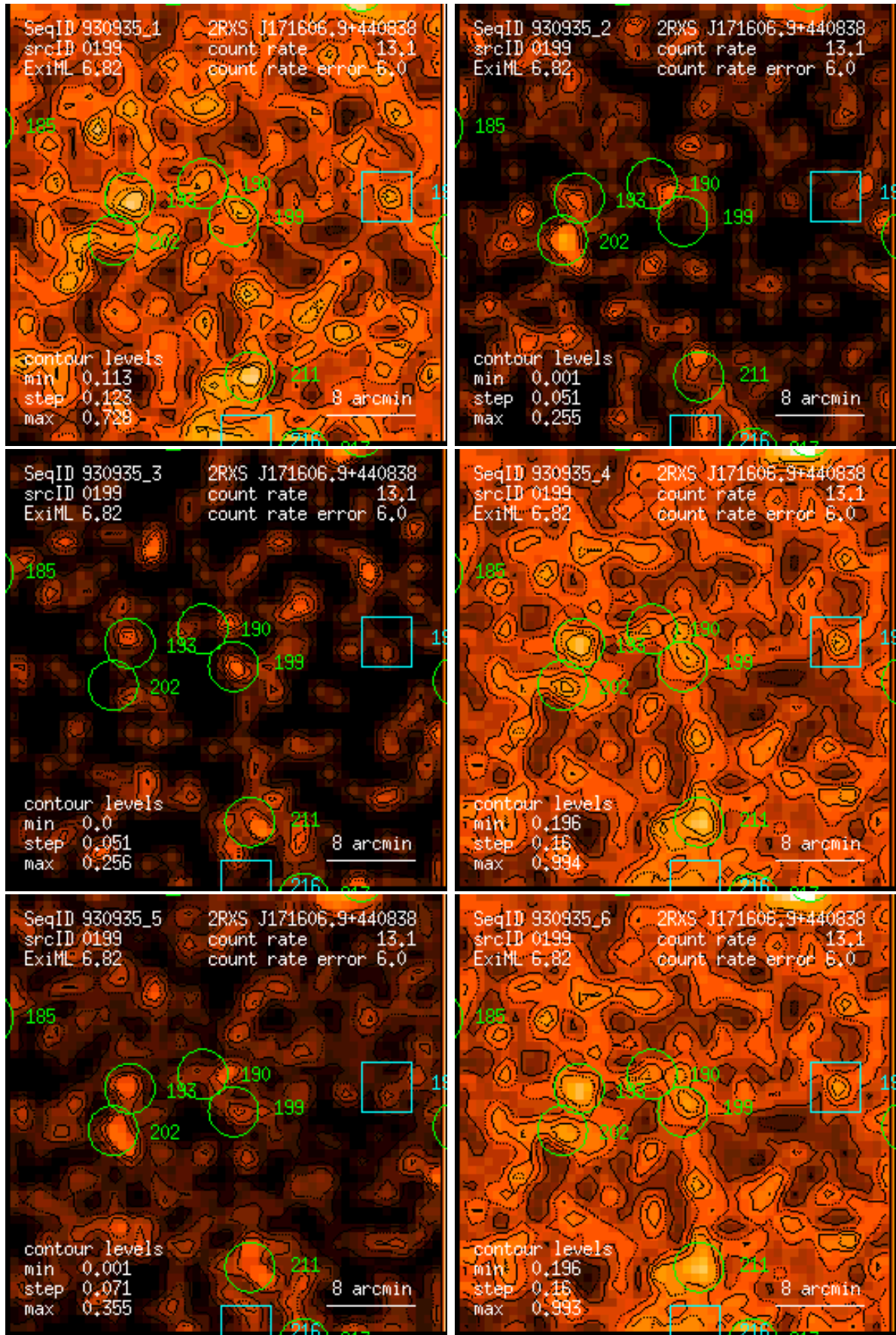
Figure 199: RASS 930935: detection 0199: band rate images, Gaussian filter: (1) PSPC channels 11 – 41, (2) 52 – 90, (3) 91 – 201, (4) 11 – 235, (5) 52 – 201, (6) 11 – 201. Broad band rates in counts/ks. Band rate contour levels in counts/ks/arcmin 2 .
