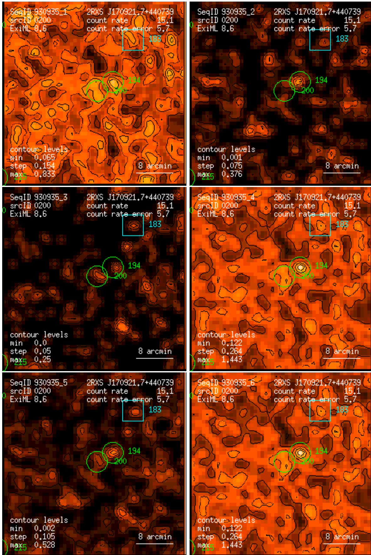
Figure 200: RASS 930935: detection 0200: band rate images, Gaussian filter: (1) PSPC channels 11 – 41, (2) 52 – 90, (3) 91 – 201, (4) 11 – 235, (5) 52 – 201, (6) 11 – 201. Broad band rates in counts/ks. Band rate contour levels in counts/ks/arcmin 2 .
