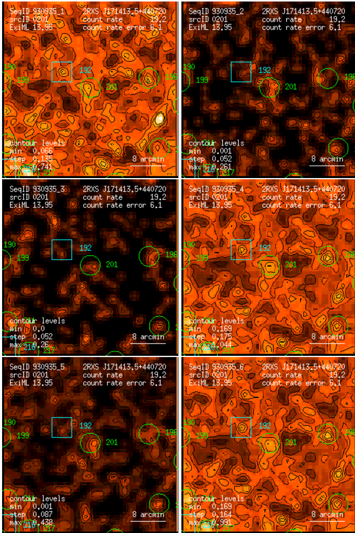
Figure 201: RASS 930935: detection 0201: band rate images, Gaussian filter: (1) PSPC channels 11 – 41, (2) 52 – 90, (3) 91 – 201, (4) 11 – 235, (5) 52 – 201, (6) 11 – 201. Broad band rates in counts/ks. Band rate contour levels in counts/ks/arcmin 2 .
