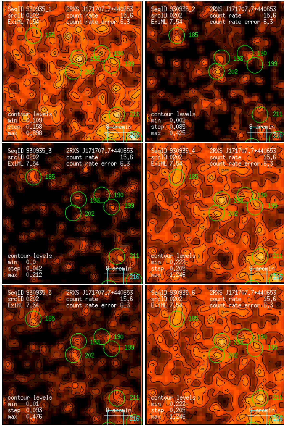
Figure 202: RASS 930935: detection 0202: band rate images, Gaussian filter: (1) PSPC channels 11 – 41, (2) 52 – 90, (3) 91 – 201, (4) 11 – 235, (5) 52 – 201, (6) 11 – 201. Broad band rates in counts/ks. Band rate contour levels in counts/ks/arcmin 2 .
