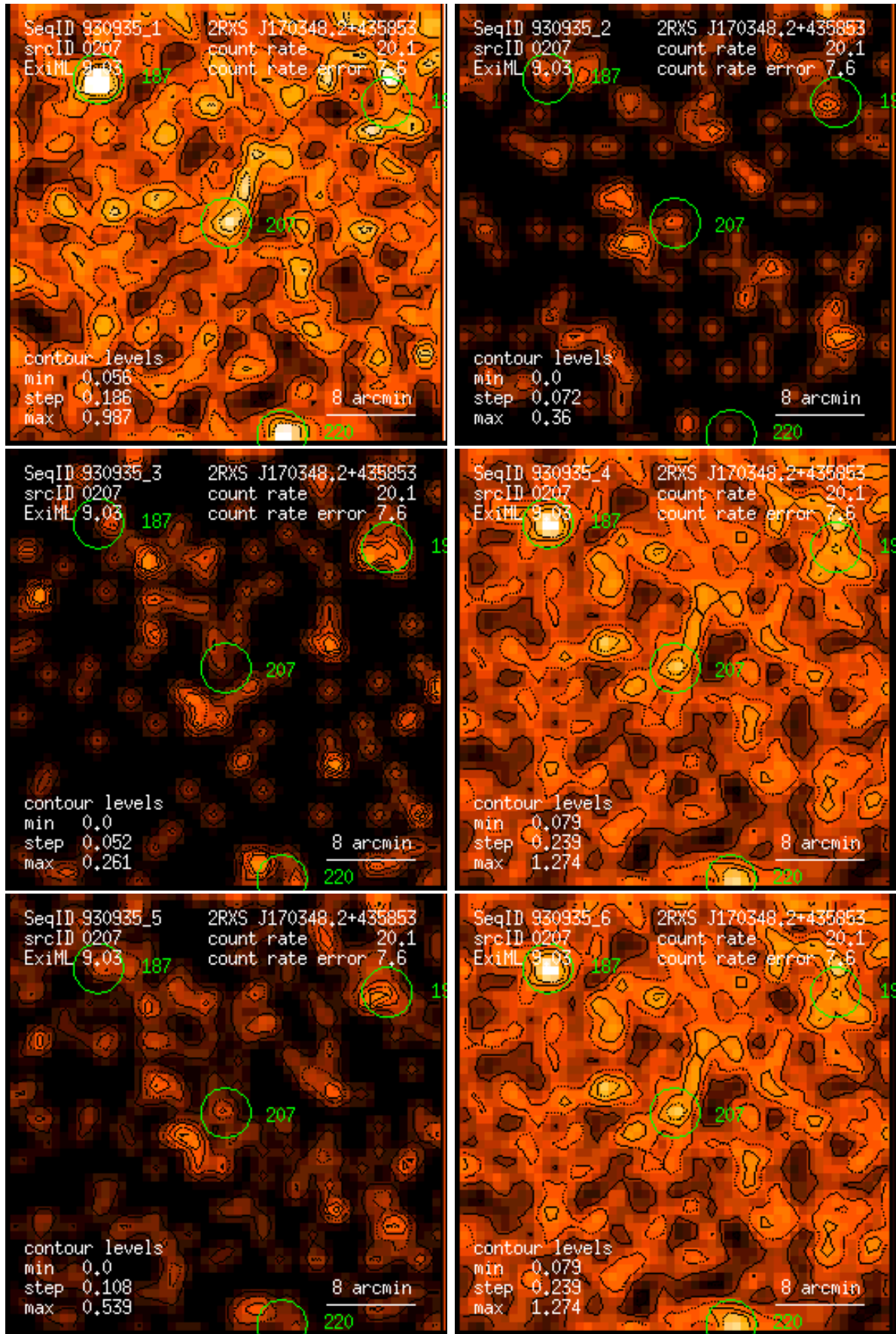
Figure 207: RASS 930935: detection 0207: band rate images, Gaussian filter: (1) PSPC channels 11 – 41, (2) 52 – 90, (3) 91 – 201, (4) 11 – 235, (5) 52 – 201, (6) 11 – 201. Broad band rates in counts/ks. Band rate contour levels in counts/ks/arcmin 2 .
