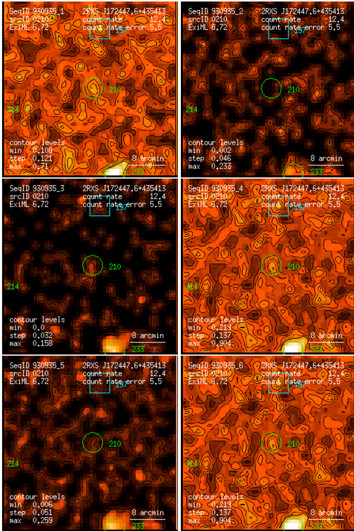
Figure 210: RASS 930935: detection 0210: band rate images, Gaussian filter: (1) PSPC channels 11 – 41, (2) 52 – 90, (3) 91 – 201, (4) 11 – 235, (5) 52 – 201, (6) 11 – 201. Broad band rates in counts/ks. Band rate contour levels in counts/ks/arcmin 2 .
