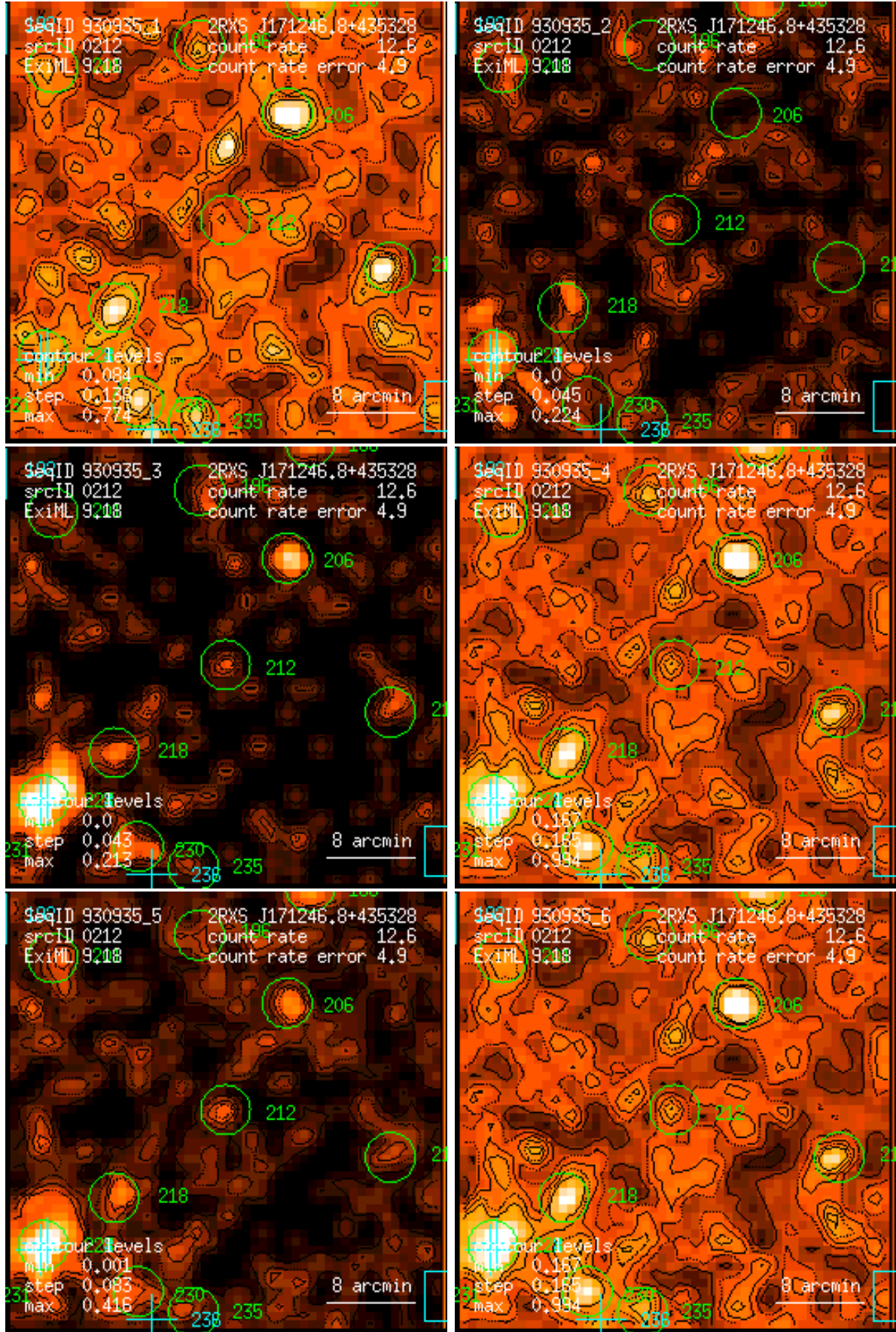
Figure 212: RASS 930935: detection 0212: band rate images, Gaussian filter: (1) PSPC channels 11 – 41, (2) 52 – 90, (3) 91 – 201, (4) 11 – 235, (5) 52 – 201, (6) 11 – 201. Broad band rates in counts/ks. Band rate contour levels in counts/ks/arcmin 2 .
