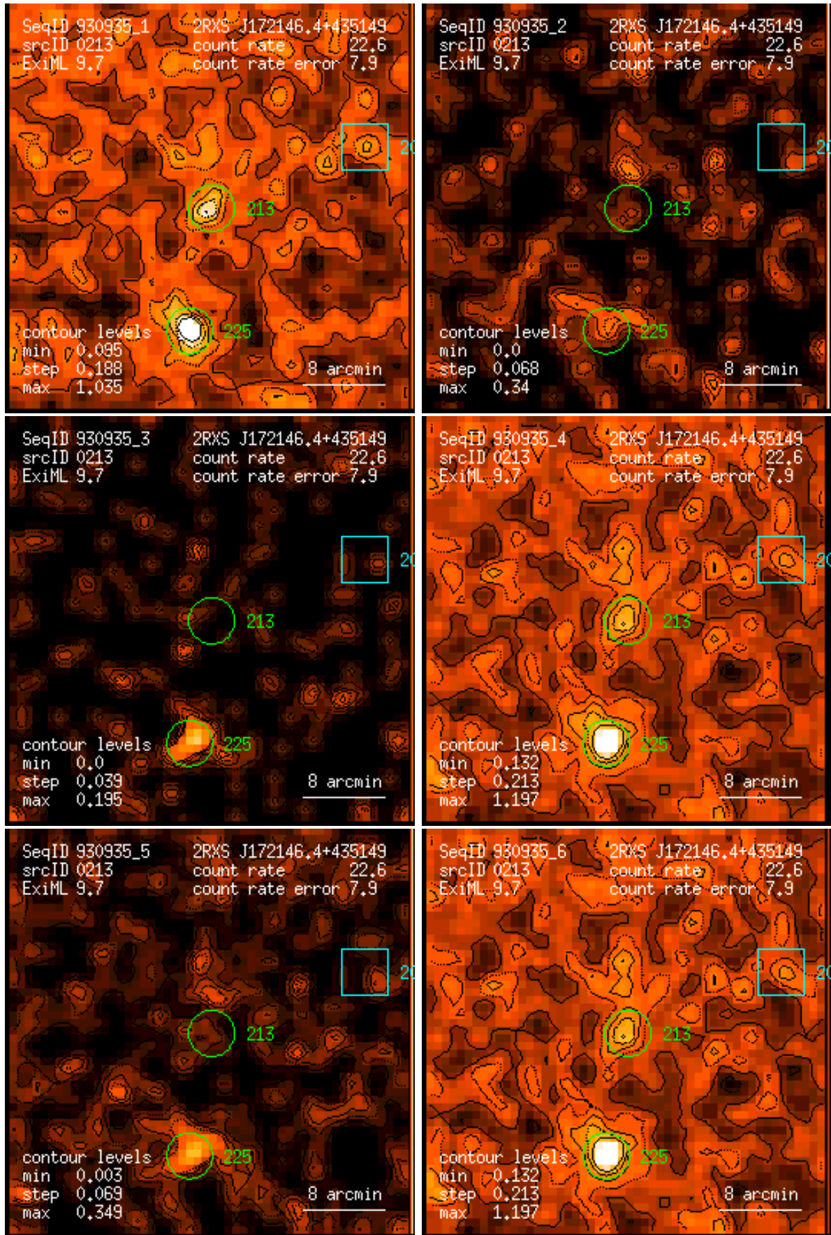
Figure 213: RASS 930935: detection 0213: band rate images, Gaussian filter: (1) PSPC channels 11 – 41, (2) 52 – 90, (3) 91 – 201, (4) 11 – 235, (5) 52 – 201, (6) 11 – 201. Broad band rates in counts/ks. Band rate contour levels in counts/ks/arcmin 2 .
