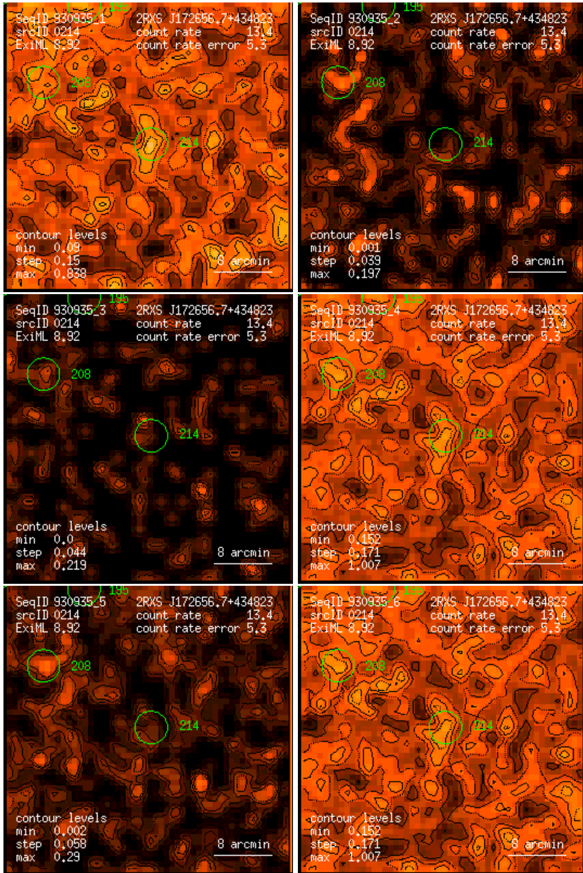
Figure 214: RASS 930935: detection 0214: band rate images, Gaussian filter: (1) PSPC channels 11 – 41, (2) 52 – 90, (3) 91 – 201, (4) 11 – 235, (5) 52 – 201, (6) 11 – 201. Broad band rates in counts/ks. Band rate contour levels in counts/ks/arcmin 2 .
