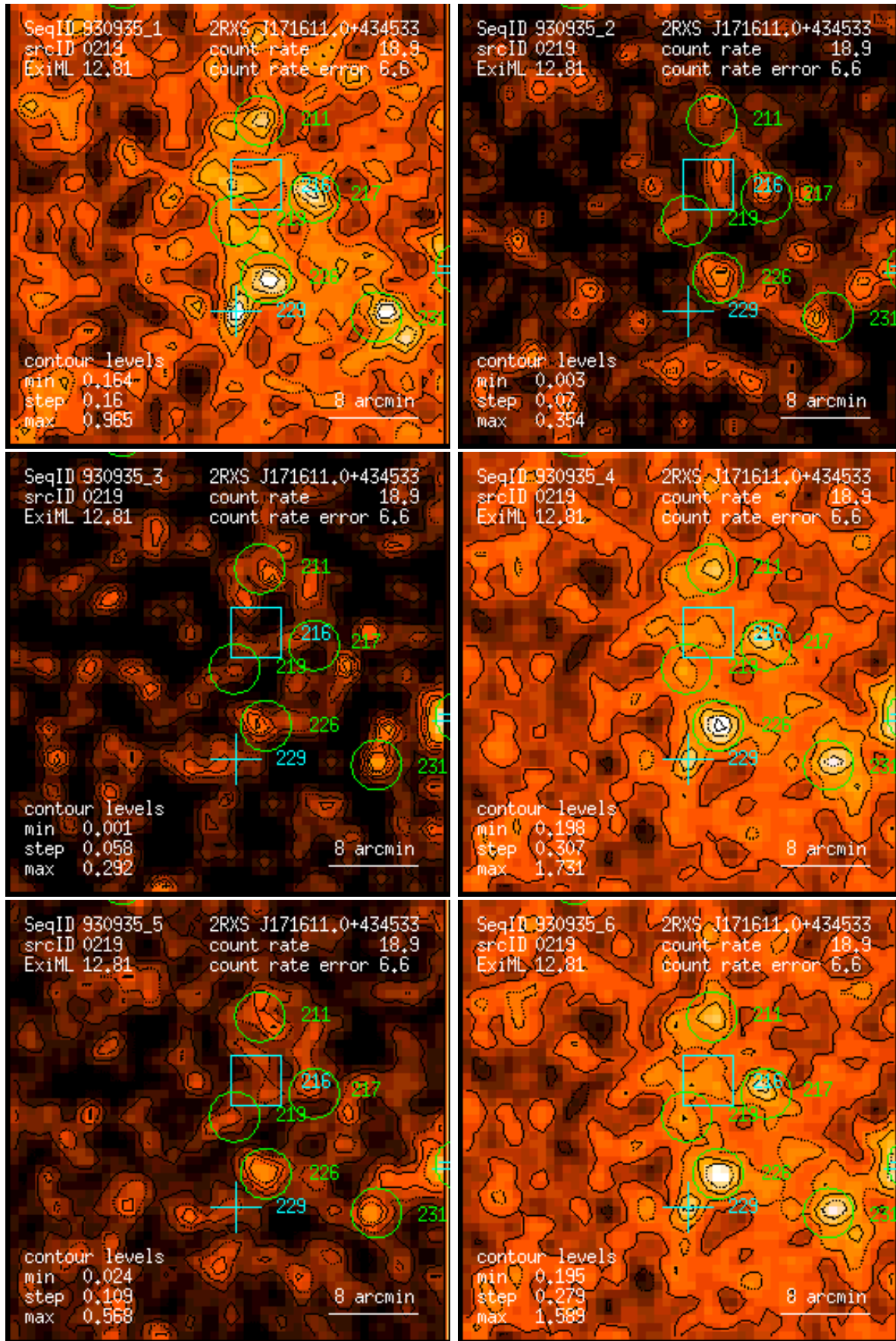
Figure 219: RASS 930935: detection 0219: band rate images, Gaussian filter: (1) PSPC channels 11 – 41, (2) 52 – 90, (3) 91 – 201, (4) 11 – 235, (5) 52 – 201, (6) 11 – 201. Broad band rates in counts/ks. Band rate contour levels in counts/ks/arcmin 2 .
