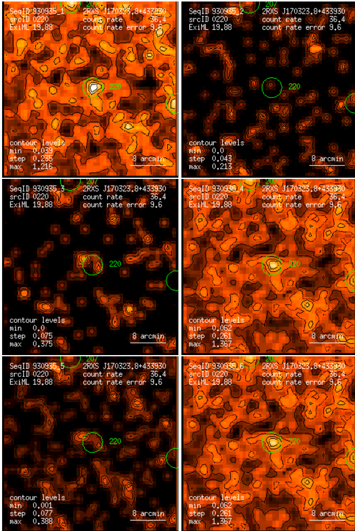
Figure 220: RASS 930935: detection 0220: band rate images, Gaussian filter: (1) PSPC channels 11 – 41, (2) 52 – 90, (3) 91 – 201, (4) 11 – 235, (5) 52 – 201, (6) 11 – 201. Broad band rates in counts/ks. Band rate contour levels in counts/ks/arcmin 2 .
