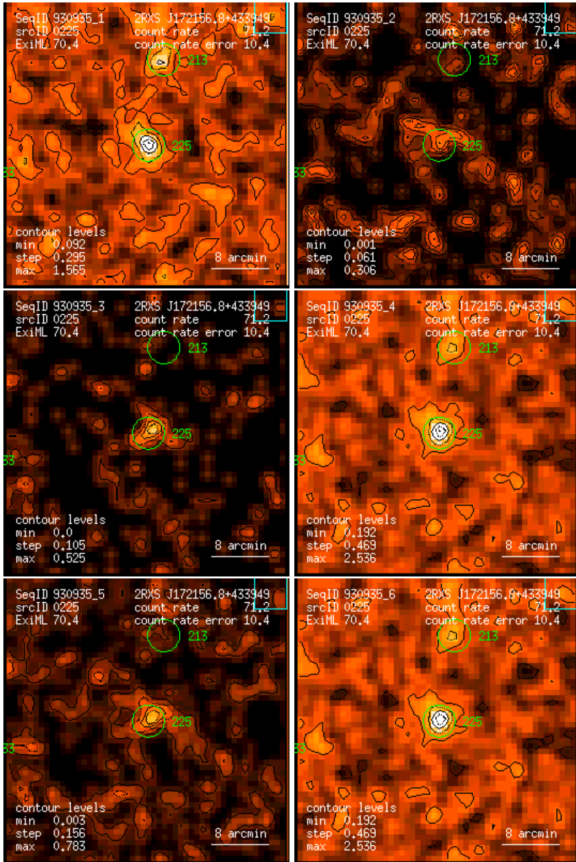
Figure 225: RASS 930935: detection 0225: band rate images, Gaussian filter: (1) PSPC channels 11 – 41, (2) 52 – 90, (3) 91 – 201, (4) 11 – 235, (5) 52 – 201, (6) 11 – 201. Broad band rates in counts/ks. Band rate contour levels in counts/ks/arcmin 2 .
