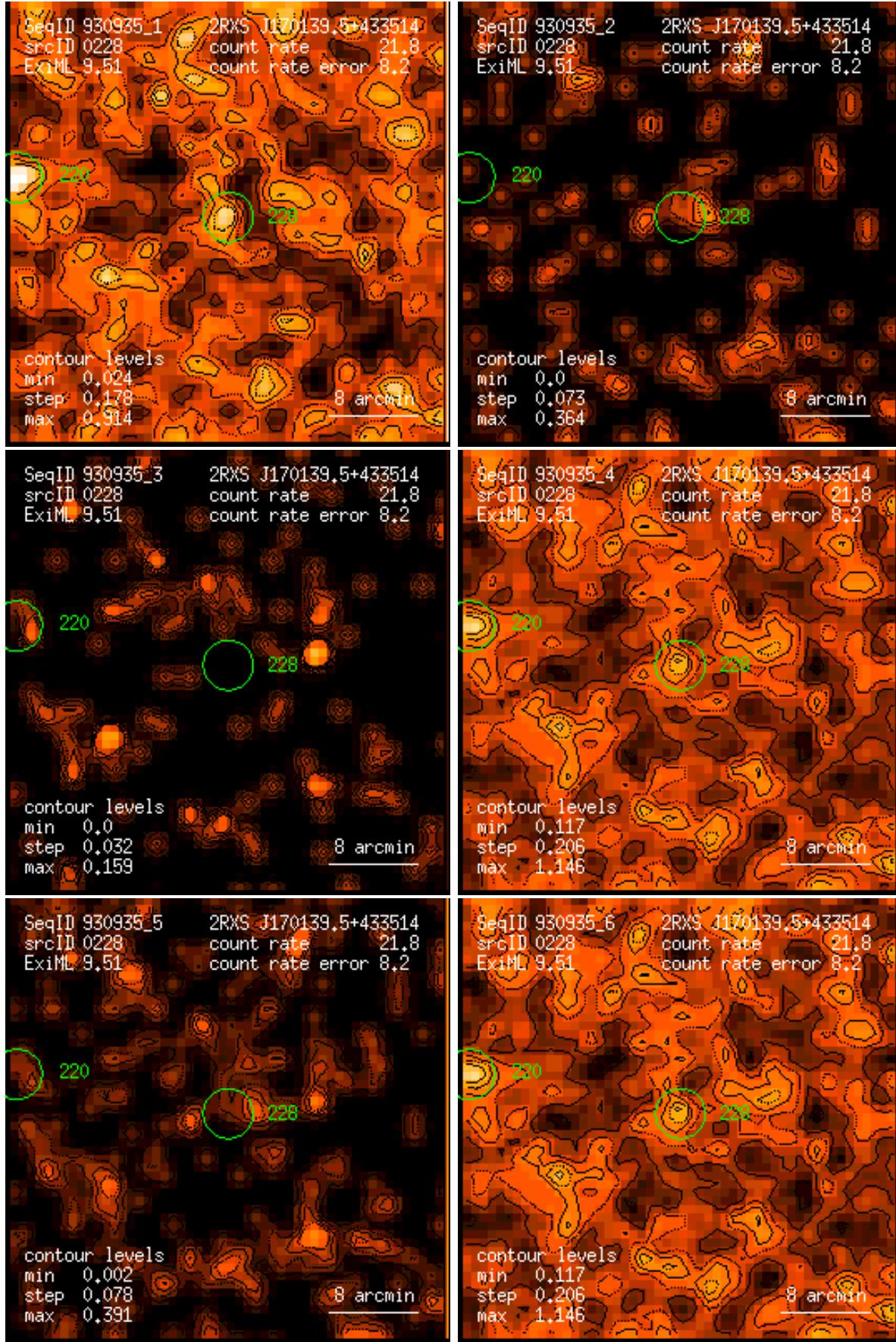
Figure 228: RASS 930935: detection 0228: band rate images, Gaussian filter: (1) PSPC channels 11 – 41, (2) 52 – 90, (3) 91 – 201, (4) 11 – 235, (5) 52 – 201, (6) 11 – 201. Broad band rates in counts/ks. Band rate contour levels in counts/ks/arcmin 2 .
