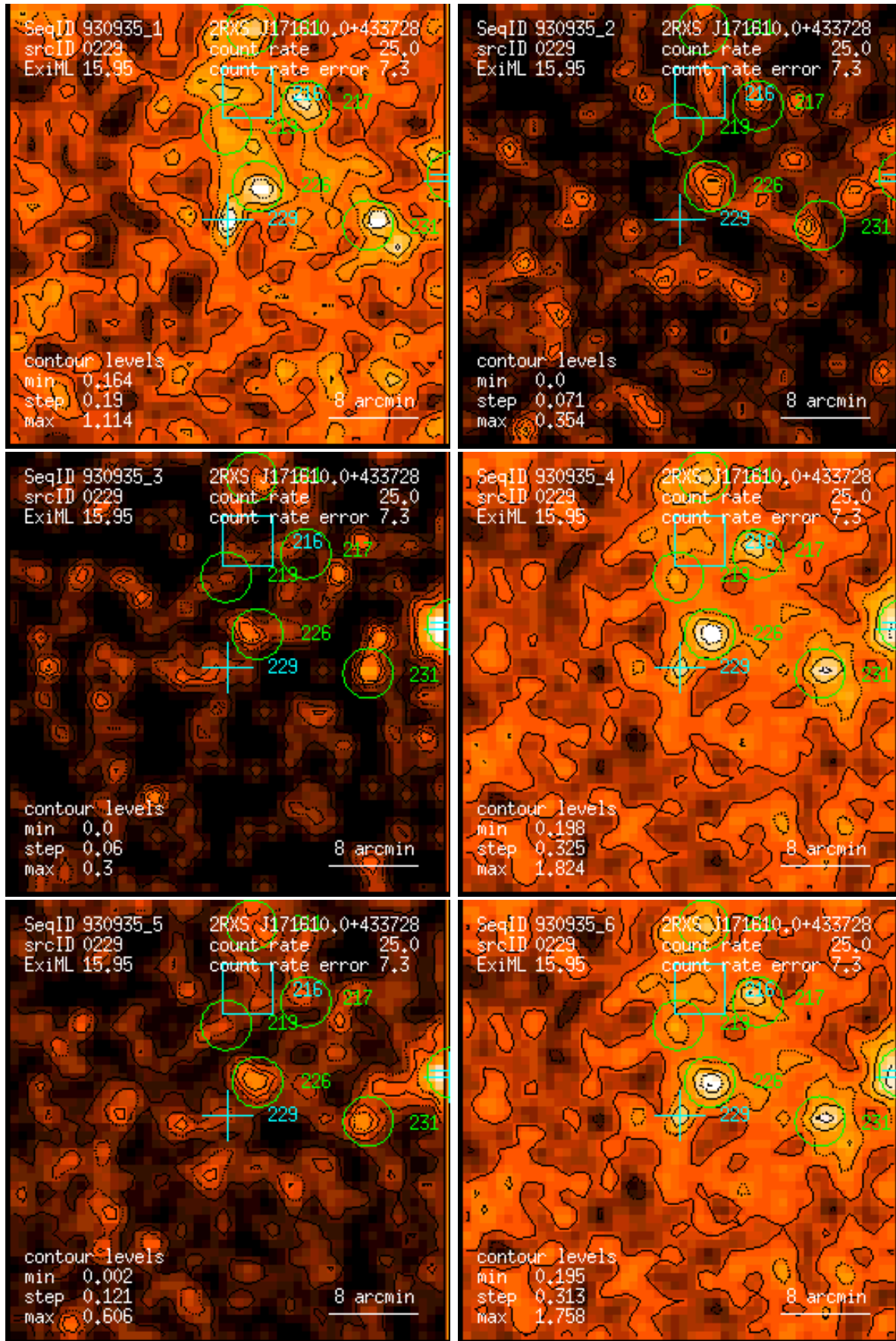
Figure 229: RASS 930935: detection 0229: band rate images, Gaussian filter: (1) PSPC channels 11 – 41, (2) 52 – 90, (3) 91 – 201, (4) 11 – 235, (5) 52 – 201, (6) 11 – 201. Broad band rates in counts/ks. Band rate contour levels in counts/ks/arcmin 2 .
