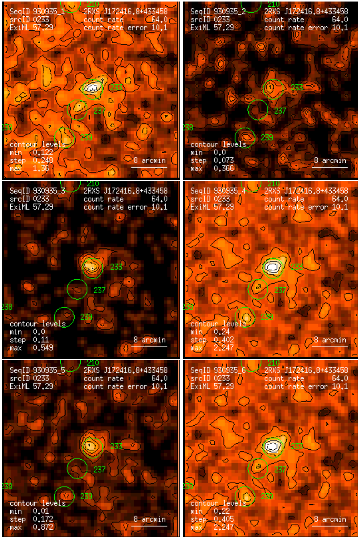
Figure 233: RASS 930935: detection 0233: band rate images, Gaussian filter: (1) PSPC channels 11 – 41, (2) 52 – 90, (3) 91 – 201, (4) 11 – 235, (5) 52 – 201, (6) 11 – 201. Broad band rates in counts/ks. Band rate contour levels in counts/ks/arcmin 2 .
